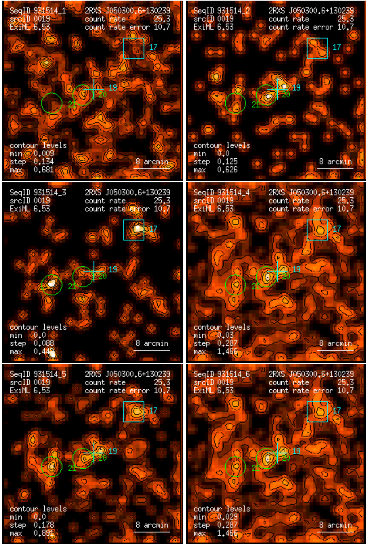
Figure 19: RASS 931514: detection 0019: band rate images, Gaussian filter: (1) PSPC channels 11 – 41, (2) 52 – 90, (3) 91 – 201, (4) 11 – 235, (5) 52 – 201, (6) 11 – 201. Broad band rates in counts/ks. Band rate contour levels in counts/ks/arcmin 2 .
