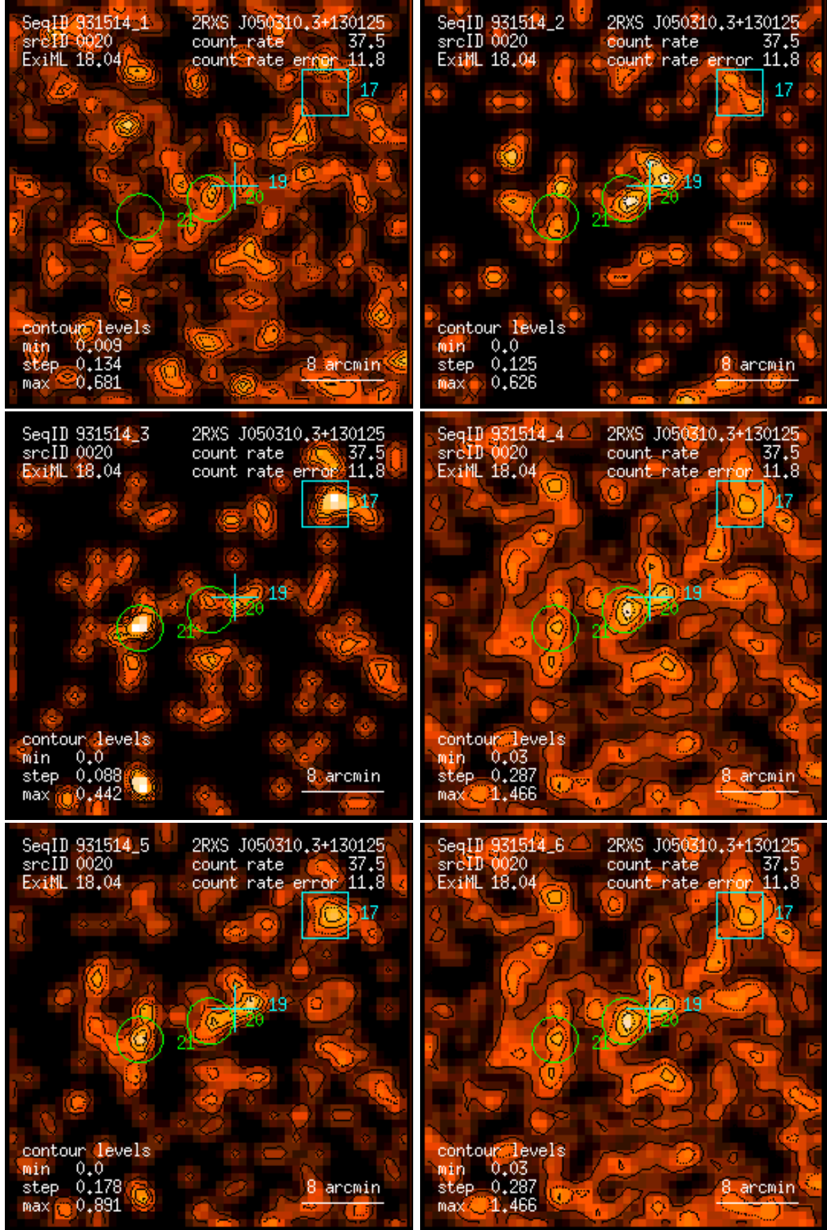
Figure 20: RASS 931514: detection 0020: band rate images, Gaussian filter: (1) PSPC channels 11 – 41, (2) 52 – 90, (3) 91 – 201, (4) 11 – 235, (5) 52 – 201, (6) 11 – 201. Broad band rates in counts/ks. Band rate contour levels in counts/ks/arcmin 2 .
