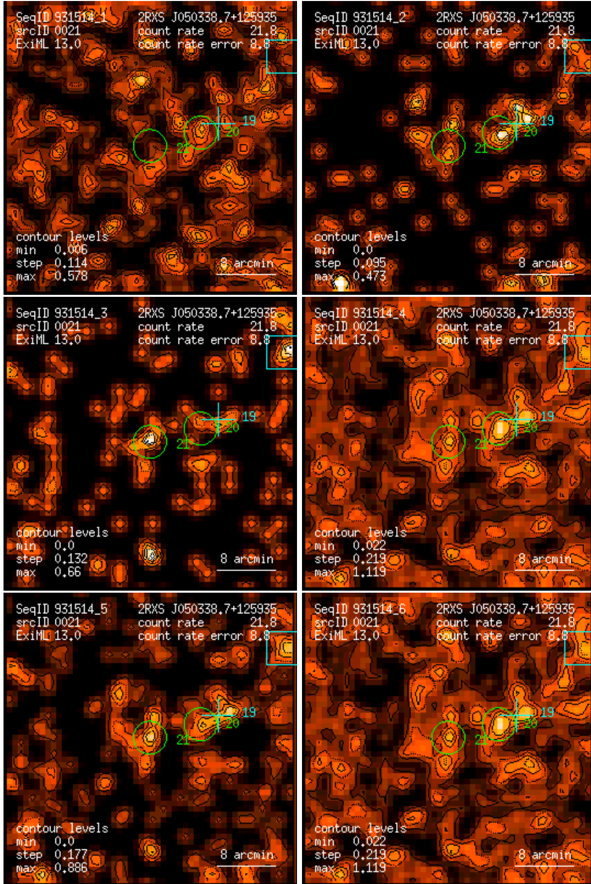
Figure 21: RASS 931514: detection 0021: band rate images, Gaussian filter: (1) PSPC channels 11 – 41, (2) 52 – 90, (3) 91 – 201, (4) 11 – 235, (5) 52 – 201, (6) 11 – 201. Broad band rates in counts/ks. Band rate contour levels in counts/ks/arcmin 2 .
