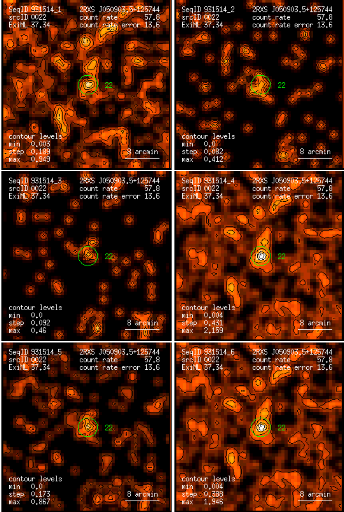
Figure 22: RASS 931514: detection 0022: band rate images, Gaussian filter: (1) PSPC channels 11 – 41, (2) 52 – 90, (3) 91 – 201, (4) 11 – 235, (5) 52 – 201, (6) 11 – 201. Broad band rates in counts/ks. Band rate contour levels in counts/ks/arcmin 2 .
