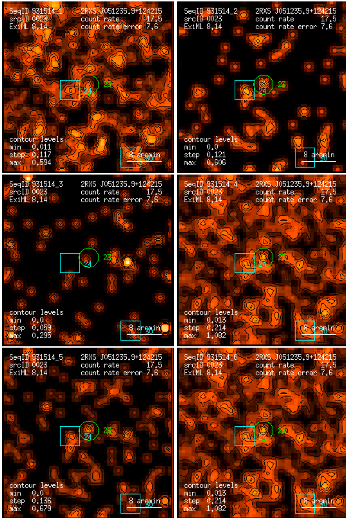
Figure 23: RASS 931514: detection 0023: band rate images, Gaussian filter: (1) PSPC channels 11 – 41, (2) 52 – 90, (3) 91 – 201, (4) 11 – 235, (5) 52 – 201, (6) 11 – 201. Broad band rates in counts/ks. Band rate contour levels in counts/ks/arcmin 2 .
