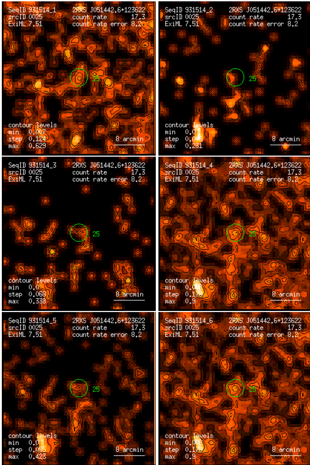
Figure 25: RASS 931514: detection 0025: band rate images, Gaussian filter: (1) PSPC channels 11 – 41, (2) 52 – 90, (3) 91 – 201, (4) 11 – 235, (5) 52 – 201, (6) 11 – 201. Broad band rates in counts/ks. Band rate contour levels in counts/ks/arcmin 2 .
