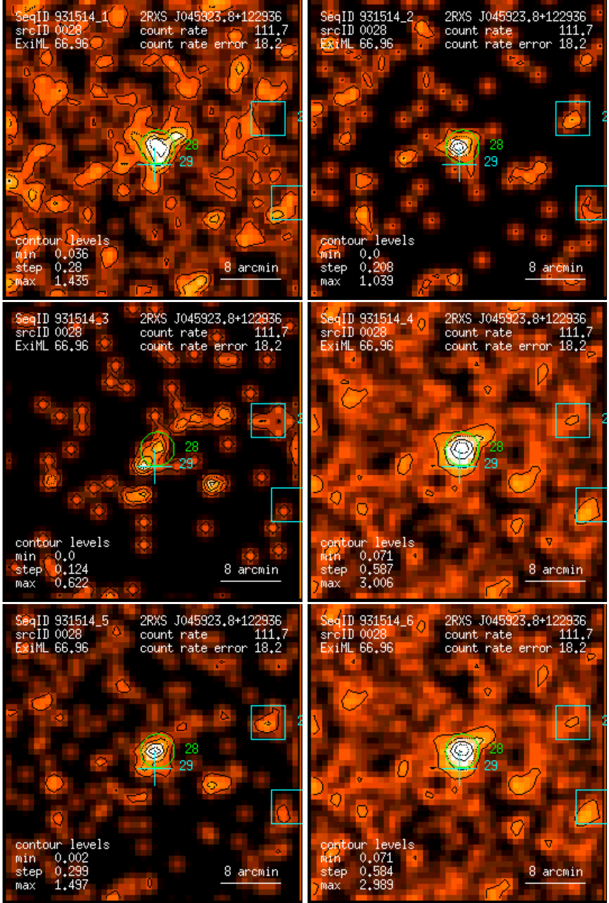
Figure 28: RASS 931514: detection 0028: band rate images, Gaussian filter: (1) PSPC channels 11 – 41, (2) 52 – 90, (3) 91 – 201, (4) 11 – 235, (5) 52 – 201, (6) 11 – 201. Broad band rates in counts/ks. Band rate contour levels in counts/ks/arcmin 2 .
