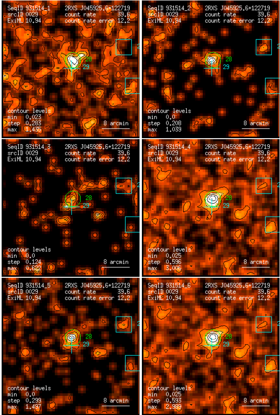
Figure 29: RASS 931514: detection 0029: band rate images, Gaussian filter: (1) PSPC channels 11 – 41, (2) 52 – 90, (3) 91 – 201, (4) 11 – 235, (5) 52 – 201, (6) 11 – 201. Broad band rates in counts/ks. Band rate contour levels in counts/ks/arcmin 2 .
