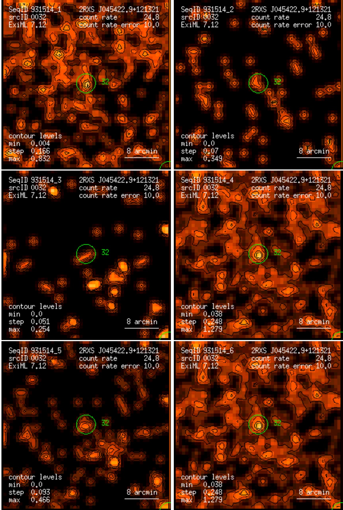
Figure 32: RASS 931514: detection 0032: band rate images, Gaussian filter: (1) PSPC channels 11 – 41, (2) 52 – 90, (3) 91 – 201, (4) 11 – 235, (5) 52 – 201, (6) 11 – 201. Broad band rates in counts/ks. Band rate contour levels in counts/ks/arcmin 2 .
