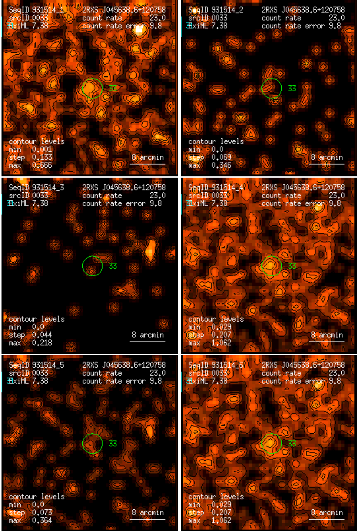
Figure 33: RASS 931514: detection 0033: band rate images, Gaussian filter: (1) PSPC channels 11 – 41, (2) 52 – 90, (3) 91 – 201, (4) 11 – 235, (5) 52 – 201, (6) 11 – 201. Broad band rates in counts/ks. Band rate contour levels in counts/ks/arcmin 2 .
