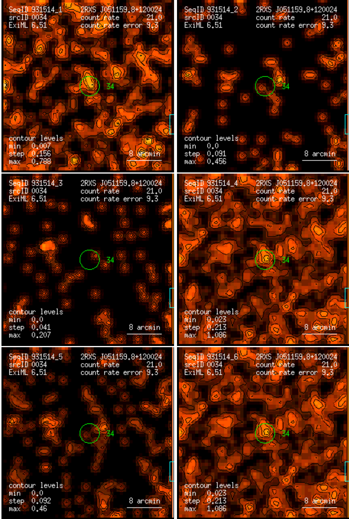
Figure 34: RASS 931514: detection 0034: band rate images, Gaussian filter: (1) PSPC channels 11 – 41, (2) 52 – 90, (3) 91 – 201, (4) 11 – 235, (5) 52 – 201, (6) 11 – 201. Broad band rates in counts/ks. Band rate contour levels in counts/ks/arcmin 2 .
