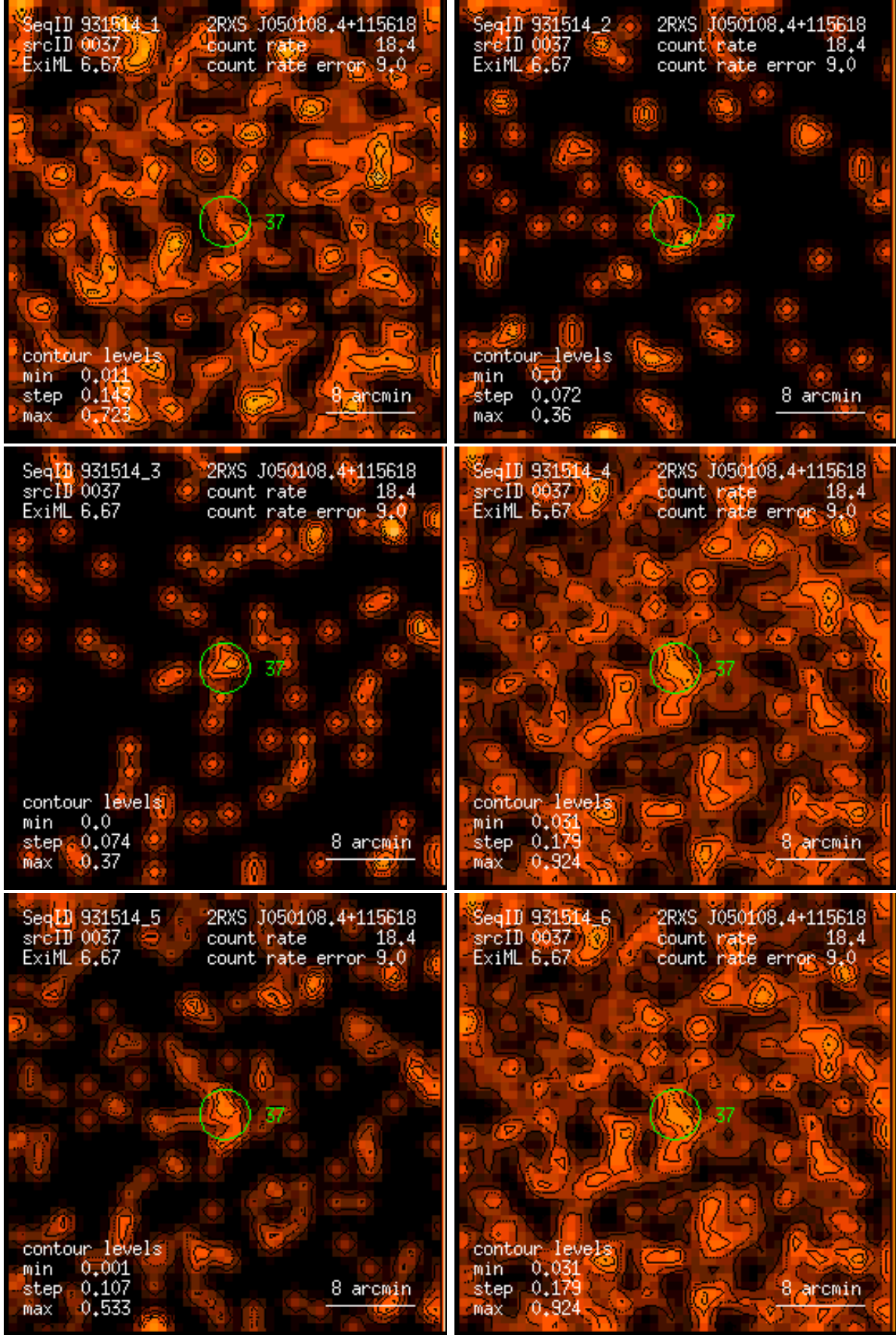
Figure 37: RASS 931514: detection 0037: band rate images, Gaussian filter: (1) PSPC channels 11 – 41, (2) 52 – 90, (3) 91 – 201, (4) 11 – 235, (5) 52 – 201, (6) 11 – 201. Broad band rates in counts/ks. Band rate contour levels in counts/ks/arcmin 2 .
