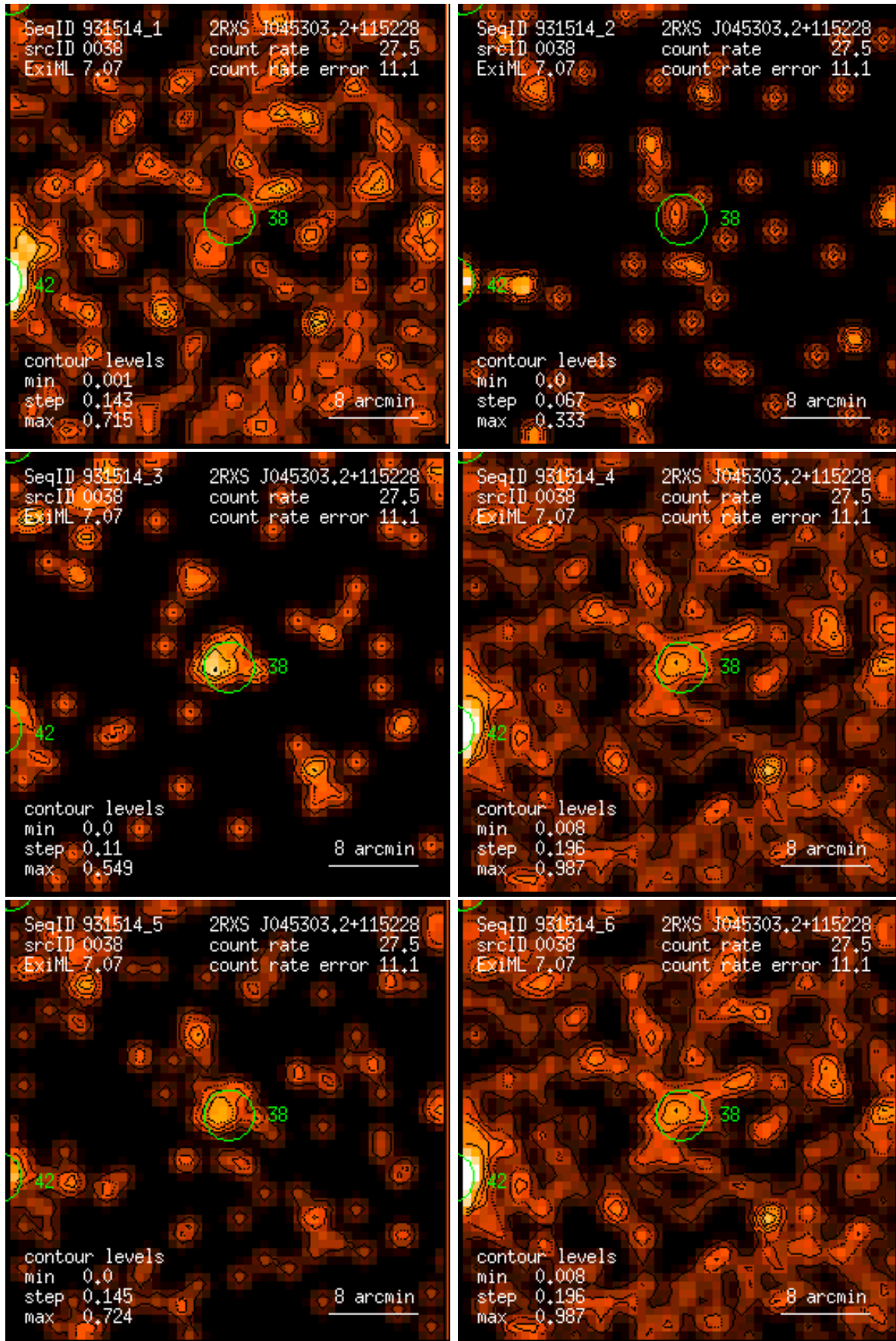
Figure 38: RASS 931514: detection 0038: band rate images, Gaussian filter: (1) PSPC channels 11 – 41, (2) 52 – 90, (3) 91 – 201, (4) 11 – 235, (5) 52 – 201, (6) 11 – 201. Broad band rates in counts/ks. Band rate contour levels in counts/ks/arcmin 2 .
