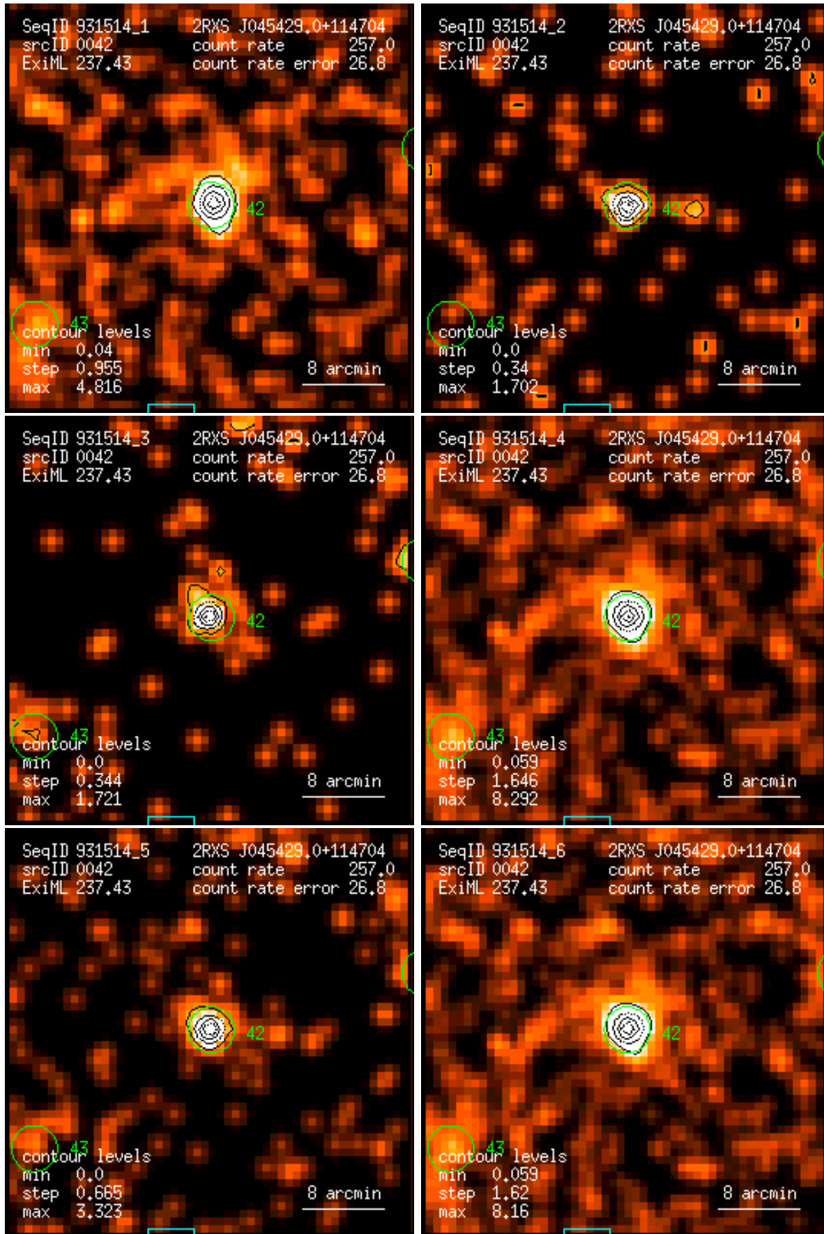
Figure 42: RASS 931514: detection 0042: band rate images, Gaussian filter: (1) PSPC channels 11 – 41, (2) 52 – 90, (3) 91 – 201, (4) 11 – 235, (5) 52 – 201, (6) 11 – 201. Broad band rates in counts/ks. Band rate contour levels in counts/ks/arcmin 2 .
