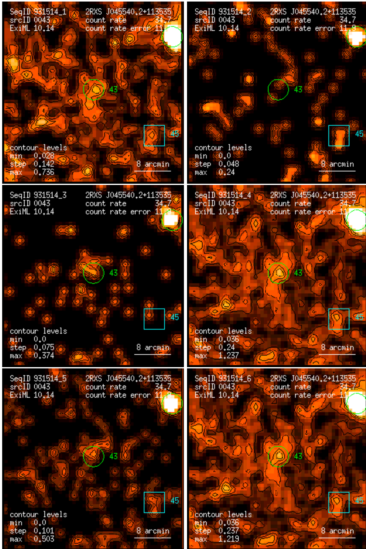
Figure 43: RASS 931514: detection 0043: band rate images, Gaussian filter: (1) PSPC channels 11 – 41, (2) 52 – 90, (3) 91 – 201, (4) 11 – 235, (5) 52 – 201, (6) 11 – 201. Broad band rates in counts/ks. Band rate contour levels in counts/ks/arcmin 2 .
