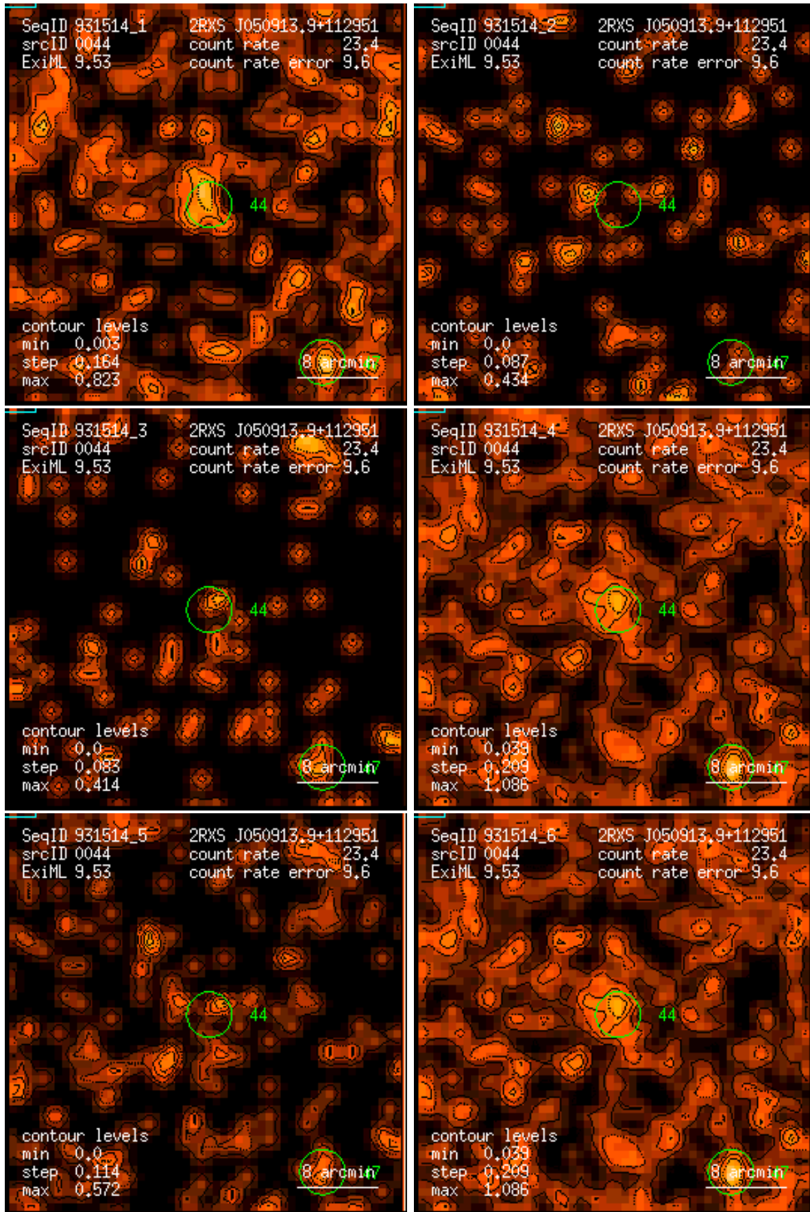
Figure 44: RASS 931514: detection 0044: band rate images, Gaussian filter: (1) PSPC channels 11 – 41, (2) 52 – 90, (3) 91 – 201, (4) 11 – 235, (5) 52 – 201, (6) 11 – 201. Broad band rates in counts/ks. Band rate contour levels in counts/ks/arcmin 2 .
