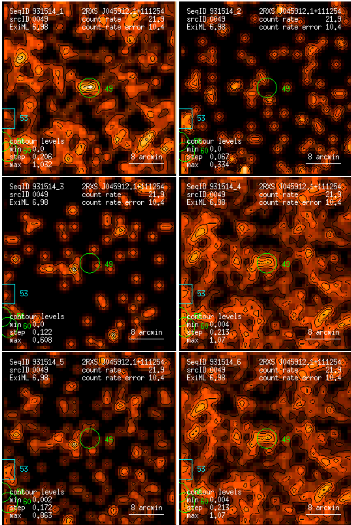
Figure 49: RASS 931514: detection 0049: band rate images, Gaussian filter: (1) PSPC channels 11 – 41, (2) 52 – 90, (3) 91 – 201, (4) 11 – 235, (5) 52 – 201, (6) 11 – 201. Broad band rates in counts/ks. Band rate contour levels in counts/ks/arcmin 2 .
