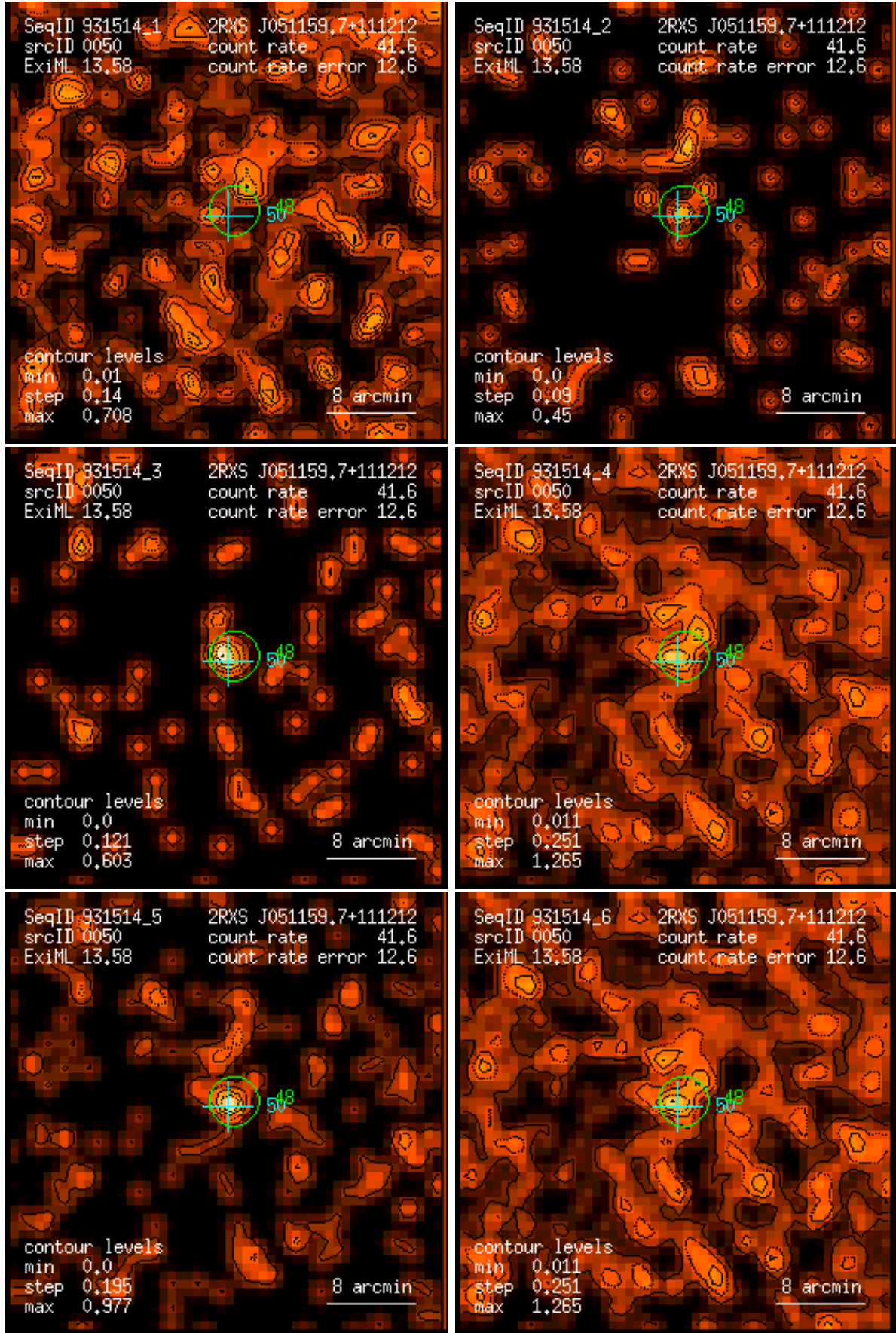
Figure 50: RASS 931514: detection 0050: band rate images, Gaussian filter: (1) PSPC channels 11 – 41, (2) 52 – 90, (3) 91 – 201, (4) 11 – 235, (5) 52 – 201, (6) 11 – 201. Broad band rates in counts/ks. Band rate contour levels in counts/ks/arcmin 2 .
