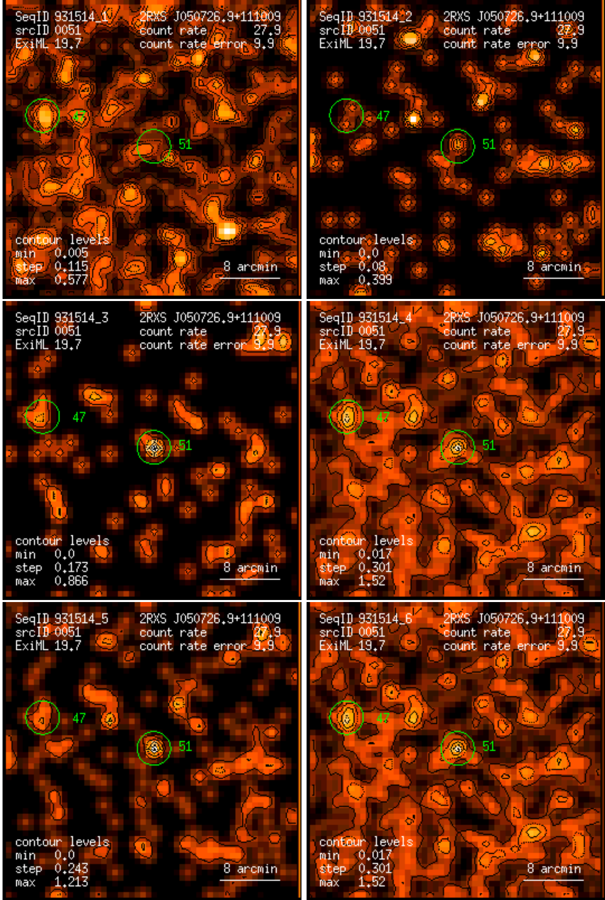
Figure 51: RASS 931514: detection 0051: band rate images, Gaussian filter: (1) PSPC channels 11 – 41, (2) 52 – 90, (3) 91 – 201, (4) 11 – 235, (5) 52 – 201, (6) 11 – 201. Broad band rates in counts/ks. Band rate contour levels in counts/ks/arcmin 2 .
