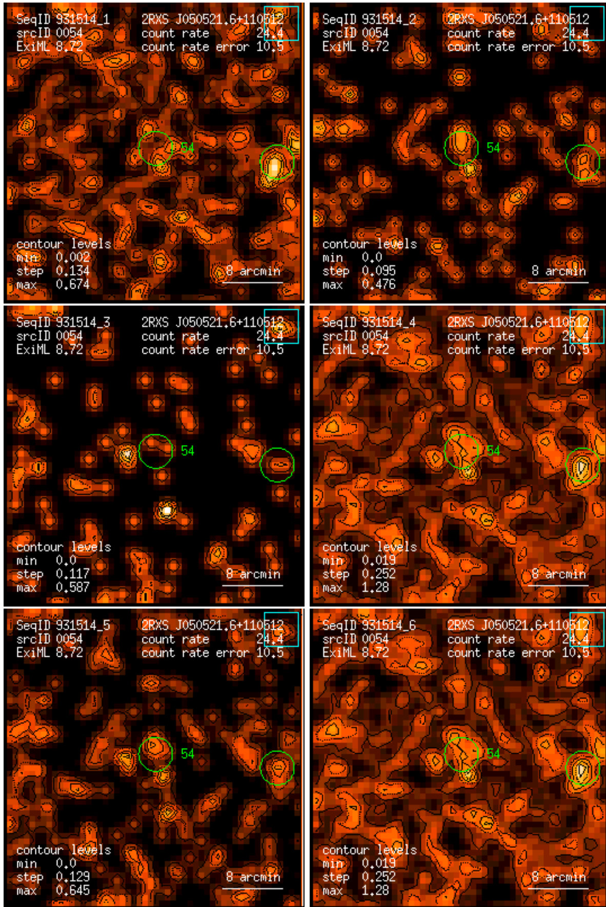
Figure 54: RASS 931514: detection 0054: band rate images, Gaussian filter: (1) PSPC channels 11 – 41, (2) 52 – 90, (3) 91 – 201, (4) 11 – 235, (5) 52 – 201, (6) 11 – 201. Broad band rates in counts/ks. Band rate contour levels in counts/ks/arcmin 2 .
