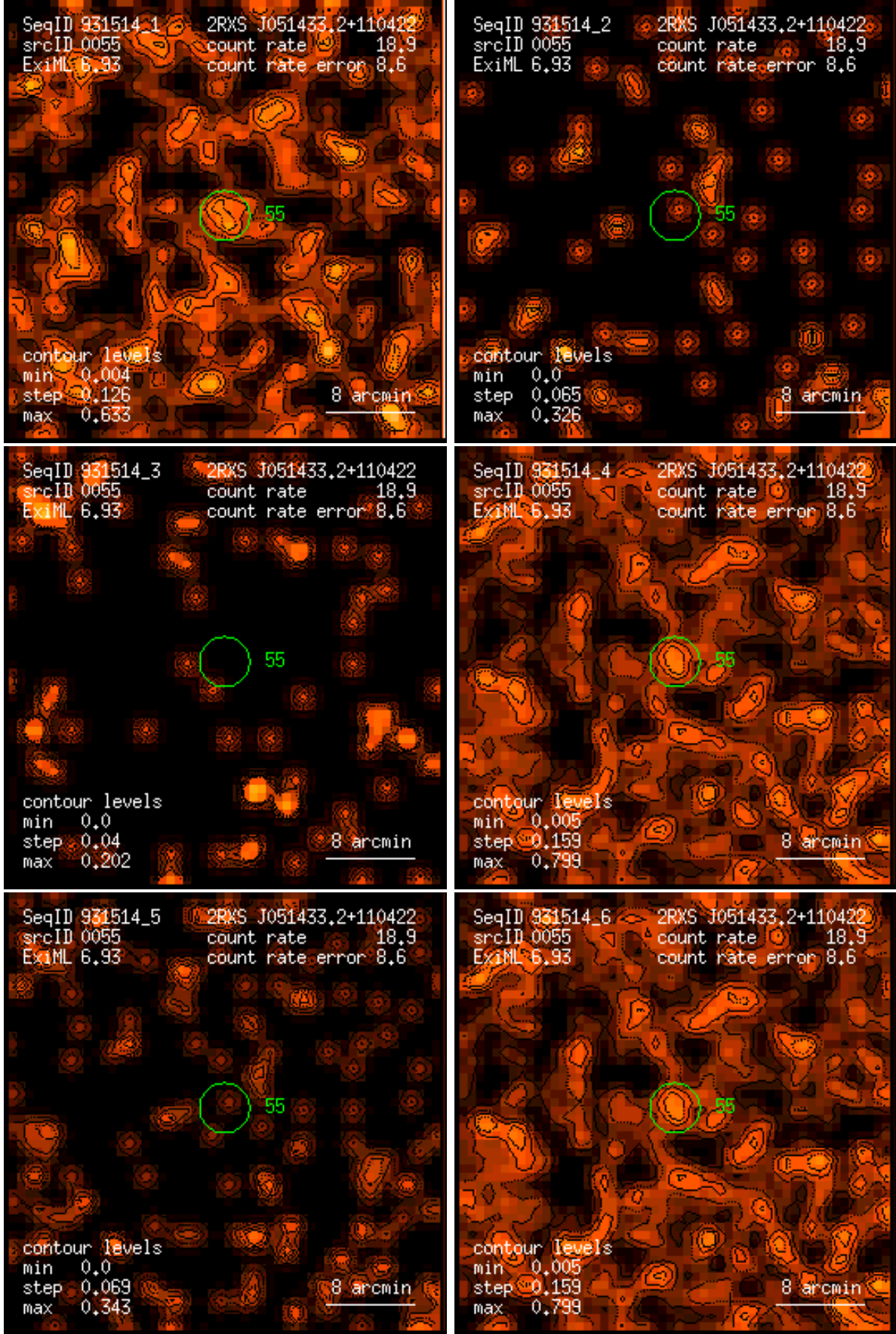
Figure 55: RASS 931514: detection 0055: band rate images, Gaussian filter: (1) PSPC channels 11 – 41, (2) 52 – 90, (3) 91 – 201, (4) 11 – 235, (5) 52 – 201, (6) 11 – 201. Broad band rates in counts/ks. Band rate contour levels in counts/ks/arcmin 2 .
