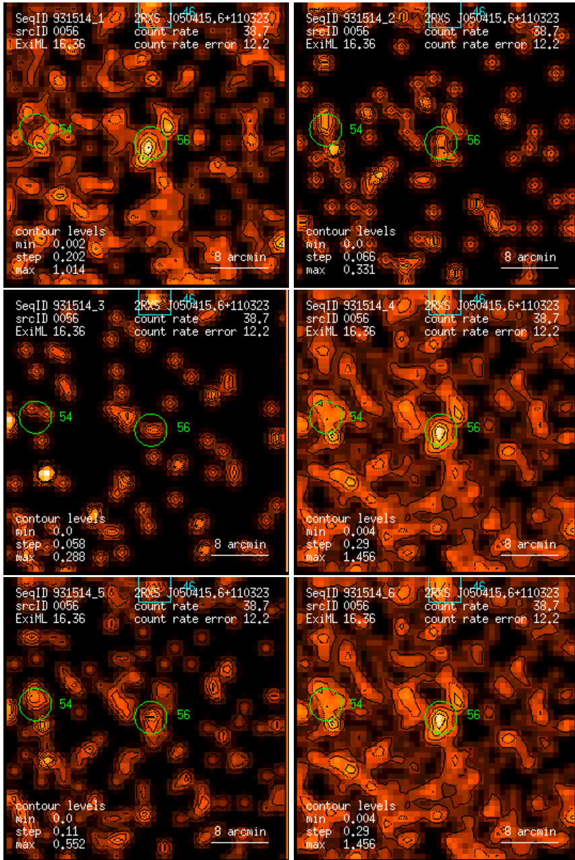
Figure 56: RASS 931514: detection 0056: band rate images, Gaussian filter: (1) PSPC channels 11 – 41, (2) 52 – 90, (3) 91 – 201, (4) 11 – 235, (5) 52 – 201, (6) 11 – 201. Broad band rates in counts/ks. Band rate contour levels in counts/ks/arcmin 2 .
