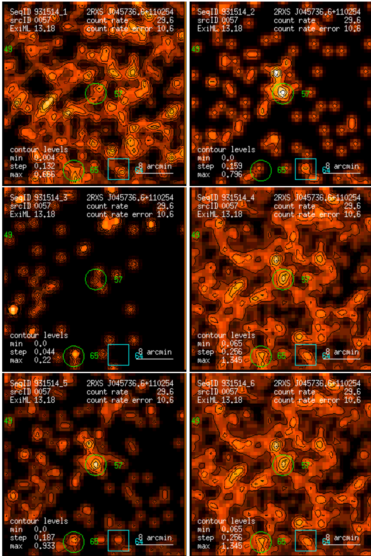
Figure 57: RASS 931514: detection 0057: band rate images, Gaussian filter: (1) PSPC channels 11 – 41, (2) 52 – 90, (3) 91 – 201, (4) 11 – 235, (5) 52 – 201, (6) 11 – 201. Broad band rates in counts/ks. Band rate contour levels in counts/ks/arcmin 2 .
