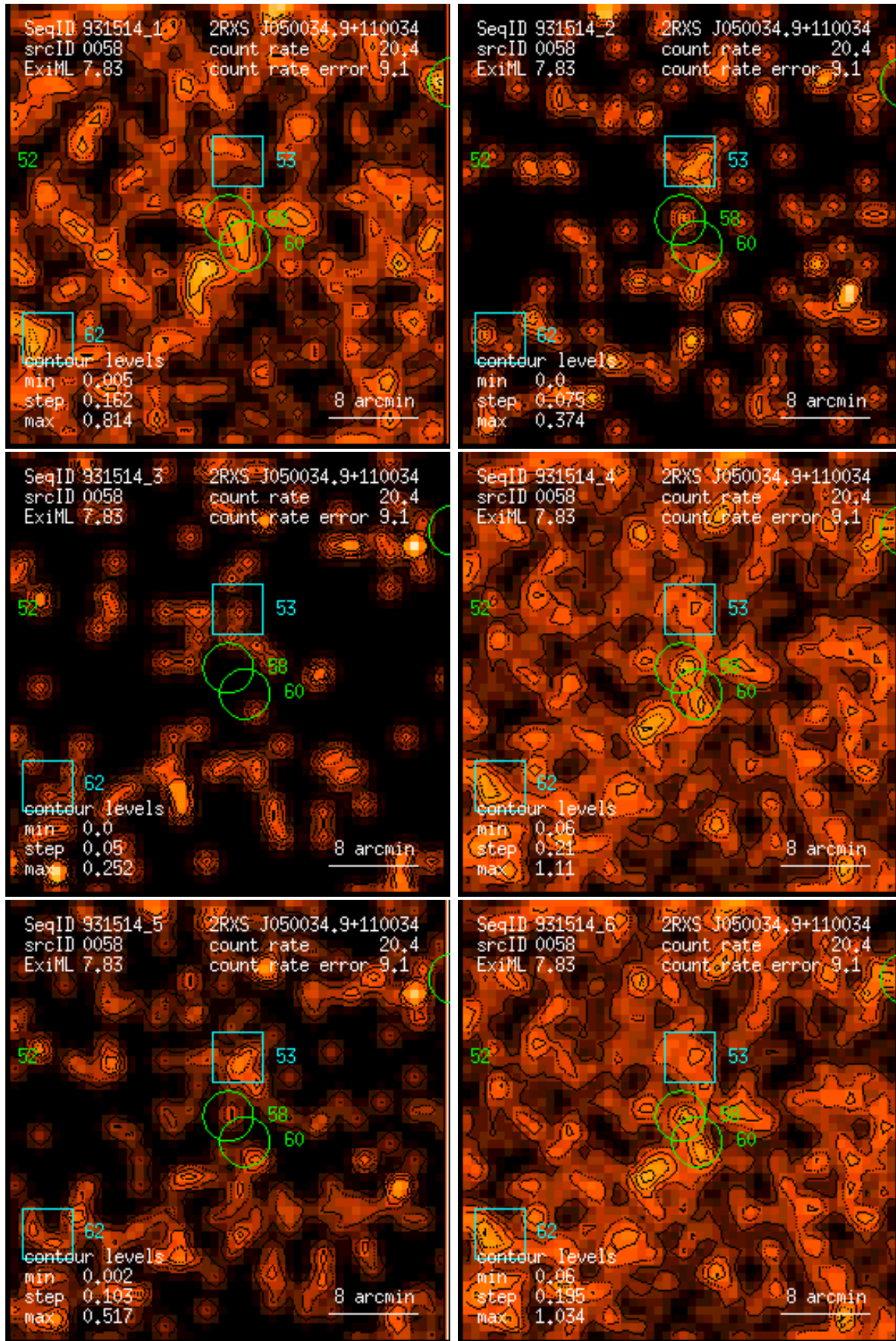
Figure 58: RASS 931514: detection 0058: band rate images, Gaussian filter: (1) PSPC channels 11 – 41, (2) 52 – 90, (3) 91 – 201, (4) 11 – 235, (5) 52 – 201, (6) 11 – 201. Broad band rates in counts/ks. Band rate contour levels in counts/ks/arcmin 2 .
