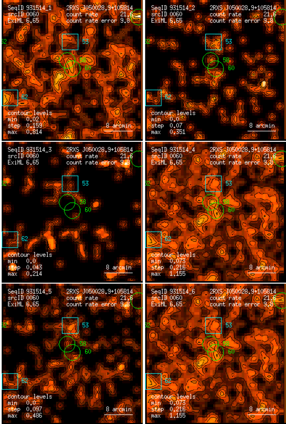
Figure 60: RASS 931514: detection 0060: band rate images, Gaussian filter: (1) PSPC channels 11 – 41, (2) 52 – 90, (3) 91 – 201, (4) 11 – 235, (5) 52 – 201, (6) 11 – 201. Broad band rates in counts/ks. Band rate contour levels in counts/ks/arcmin 2 .
