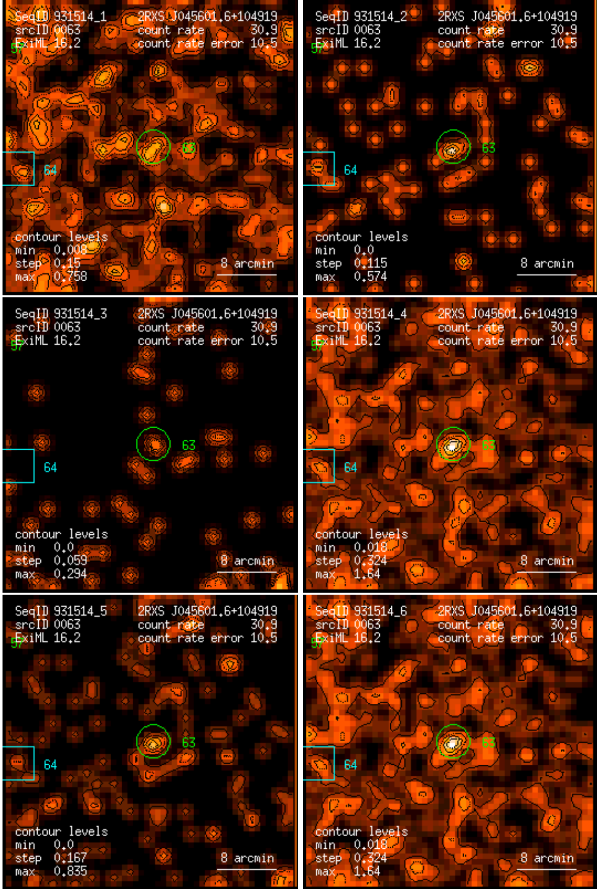
Figure 63: RASS 931514: detection 0063: band rate images, Gaussian filter: (1) PSPC channels 11 – 41, (2) 52 – 90, (3) 91 – 201, (4) 11 – 235, (5) 52 – 201, (6) 11 – 201. Broad band rates in counts/ks. Band rate contour levels in counts/ks/arcmin 2 .
