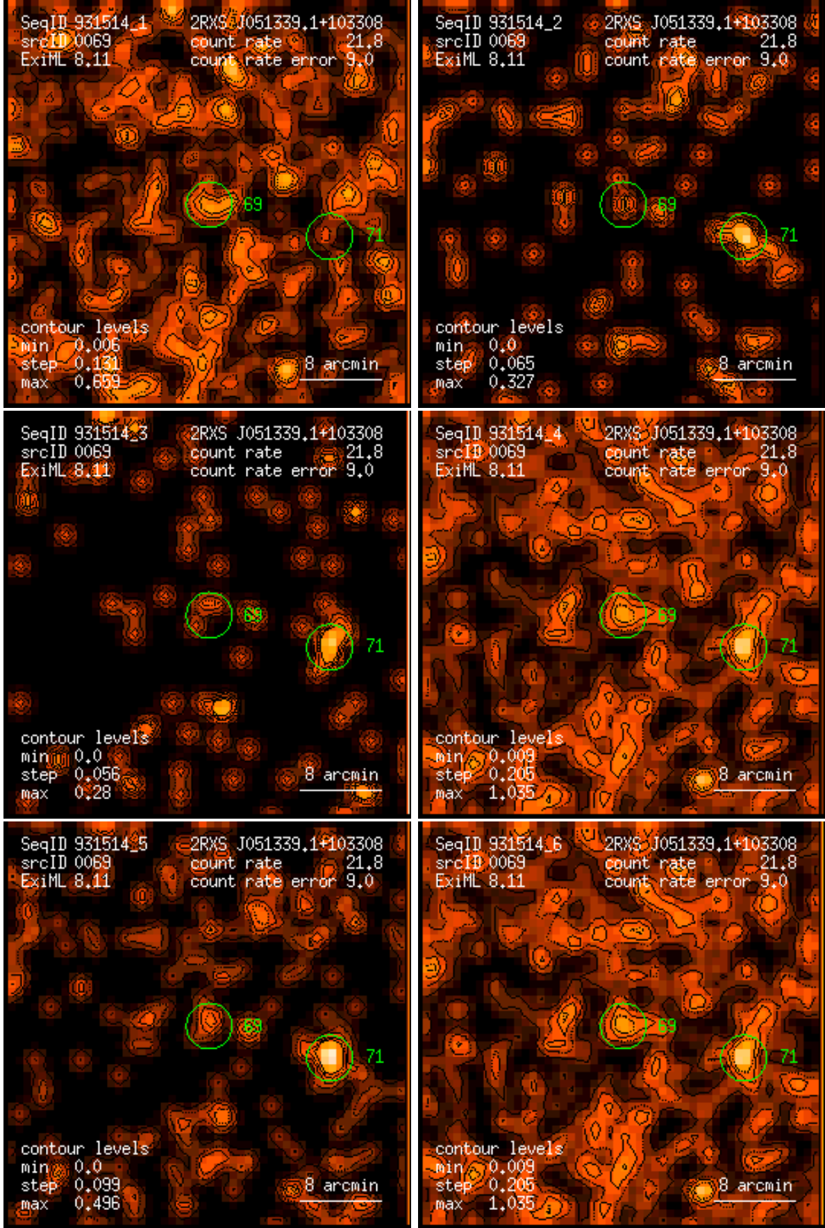
Figure 69: RASS 931514: detection 0069: band rate images, Gaussian filter: (1) PSPC channels 11 – 41, (2) 52 – 90, (3) 91 – 201, (4) 11 – 235, (5) 52 – 201, (6) 11 – 201. Broad band rates in counts/ks. Band rate contour levels in counts/ks/arcmin 2 .
