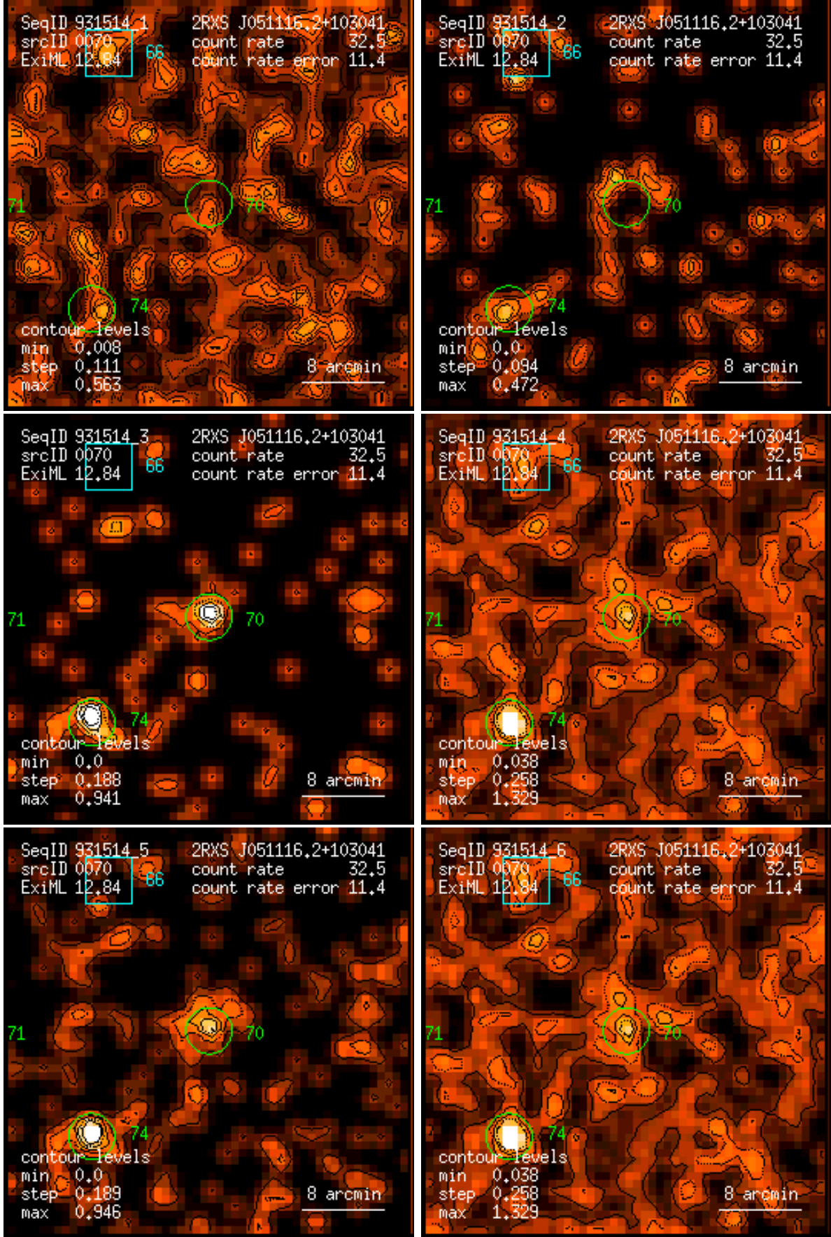
Figure 70: RASS 931514: detection 0070: band rate images, Gaussian filter: (1) PSPC channels 11 – 41, (2) 52 – 90, (3) 91 – 201, (4) 11 – 235, (5) 52 – 201, (6) 11 – 201. Broad band rates in counts/ks. Band rate contour levels in counts/ks/arcmin 2 .
