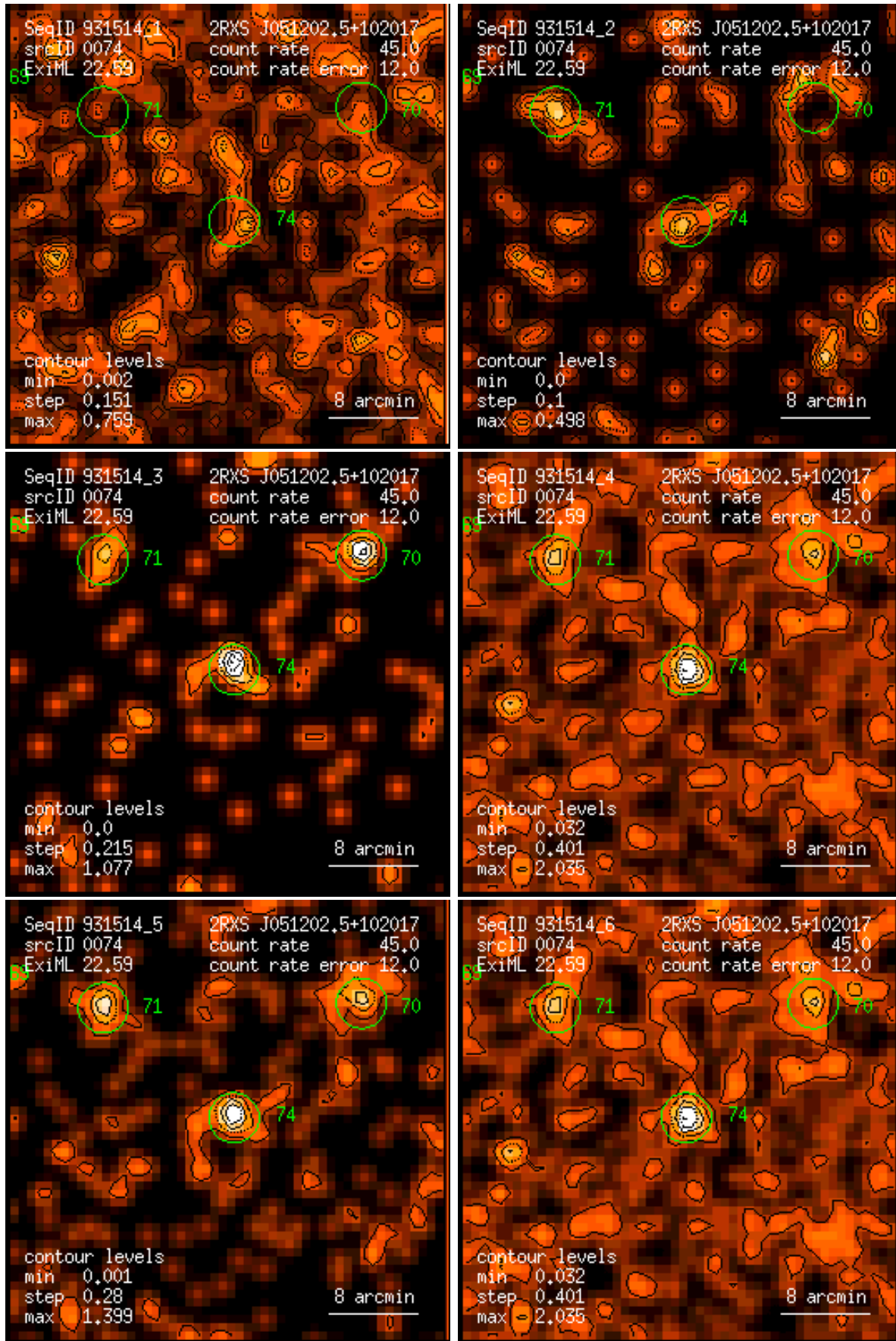
Figure 74: RASS 931514: detection 0074: band rate images, Gaussian filter: (1) PSPC channels 11 – 41, (2) 52 – 90, (3) 91 – 201, (4) 11 – 235, (5) 52 – 201, (6) 11 – 201. Broad band rates in counts/ks. Band rate contour levels in counts/ks/arcmin 2 .
