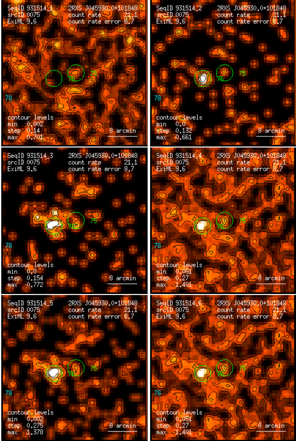
Figure 75: RASS 931514: detection 0075: band rate images, Gaussian filter: (1) PSPC channels 11 – 41, (2) 52 – 90, (3) 91 – 201, (4) 11 – 235, (5) 52 – 201, (6) 11 – 201. Broad band rates in counts/ks. Band rate contour levels in counts/ks/arcmin 2 .
