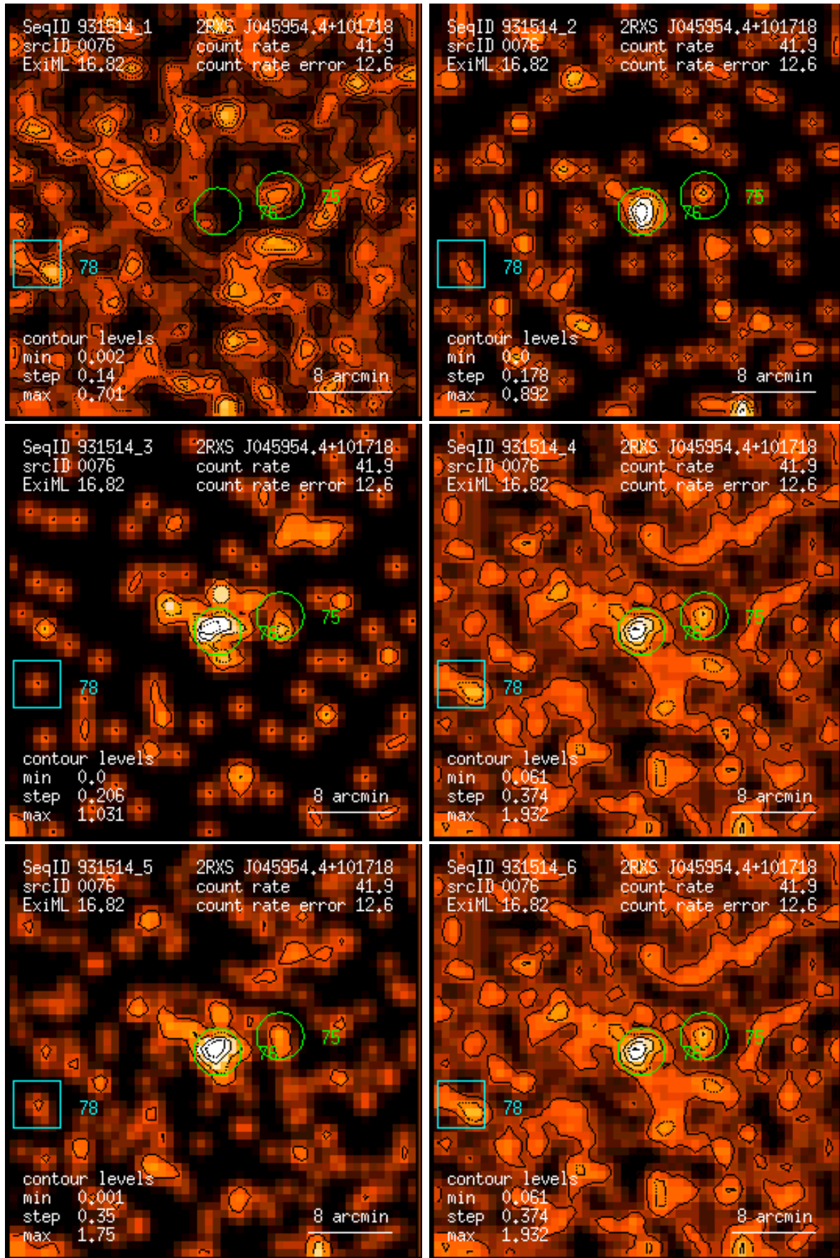
Figure 76: RASS 931514: detection 0076: band rate images, Gaussian filter: (1) PSPC channels 11 – 41, (2) 52 – 90, (3) 91 – 201, (4) 11 – 235, (5) 52 – 201, (6) 11 – 201. Broad band rates in counts/ks. Band rate contour levels in counts/ks/arcmin 2 .
