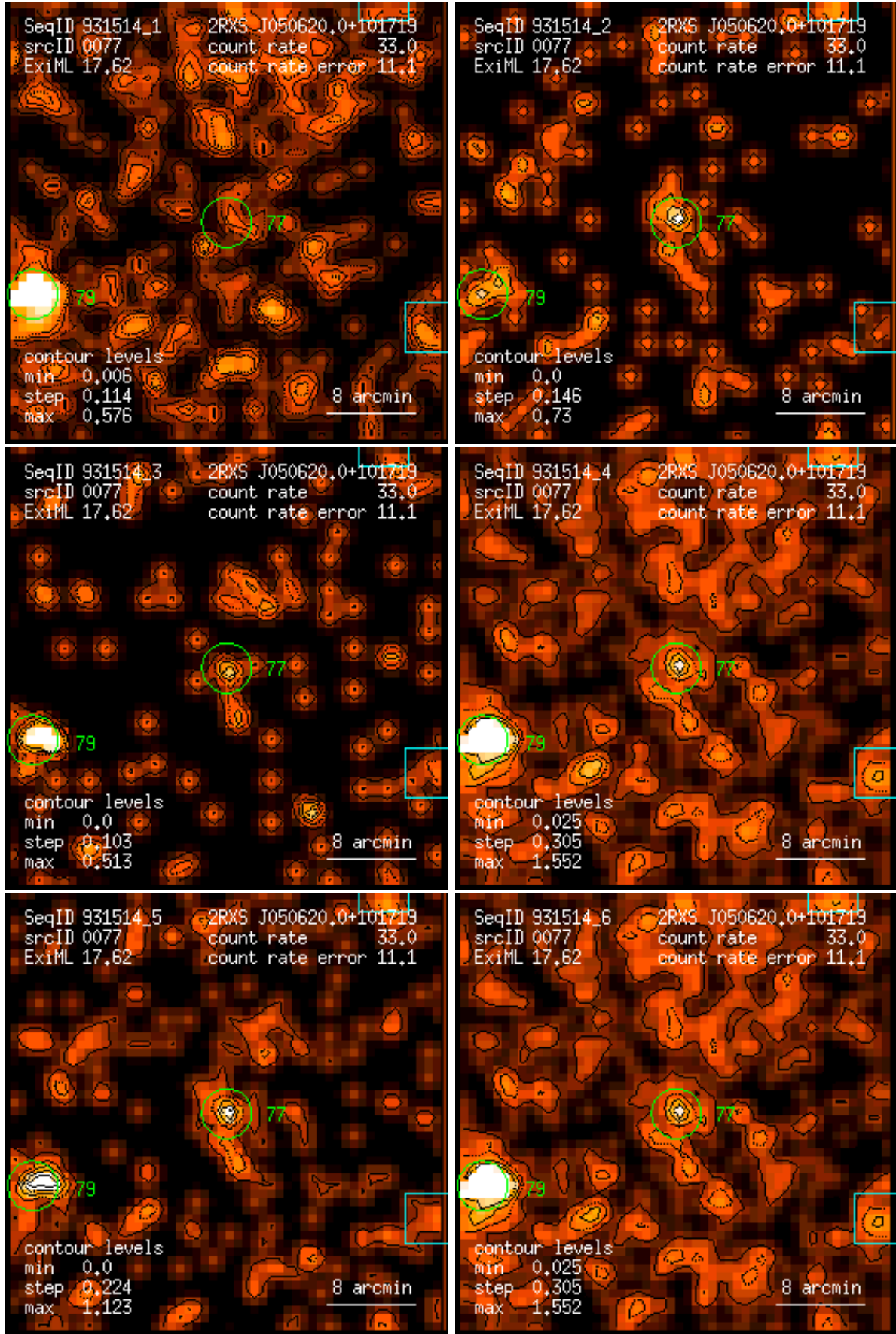
Figure 77: RASS 931514: detection 0077: band rate images, Gaussian filter: (1) PSPC channels 11 – 41, (2) 52 – 90, (3) 91 – 201, (4) 11 – 235, (5) 52 – 201, (6) 11 – 201. Broad band rates in counts/ks. Band rate contour levels in counts/ks/arcmin 2 .
