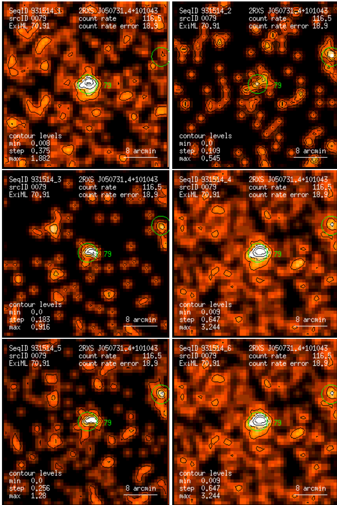
Figure 79: RASS 931514: detection 0079: band rate images, Gaussian filter: (1) PSPC channels 11 – 41, (2) 52 – 90, (3) 91 – 201, (4) 11 – 235, (5) 52 – 201, (6) 11 – 201. Broad band rates in counts/ks. Band rate contour levels in counts/ks/arcmin 2 .
