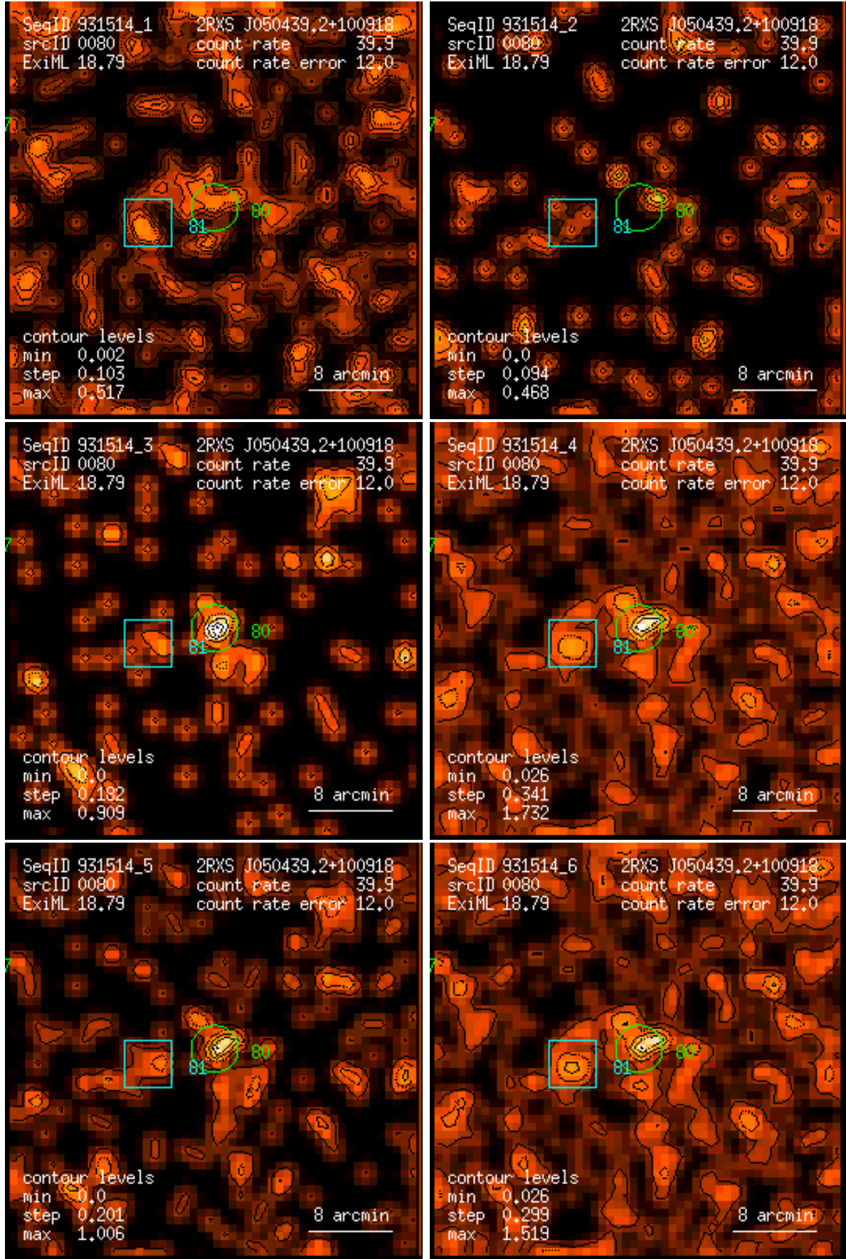
Figure 80: RASS 931514: detection 0080: band rate images, Gaussian filter: (1) PSPC channels 11 – 41, (2) 52 – 90, (3) 91 – 201, (4) 11 – 235, (5) 52 – 201, (6) 11 – 201. Broad band rates in counts/ks. Band rate contour levels in counts/ks/arcmin 2 .
