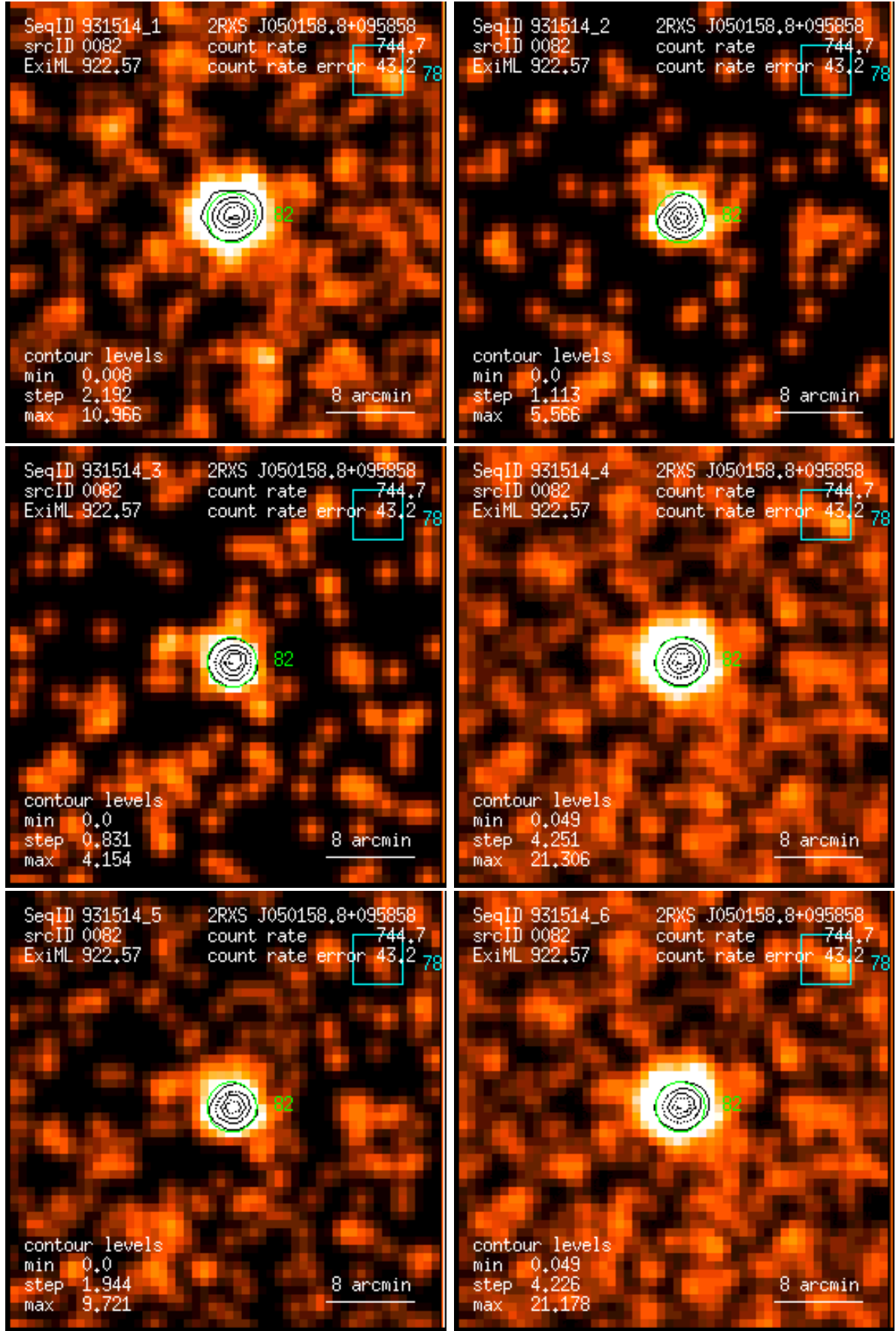
Figure 82: RASS 931514: detection 0082: band rate images, Gaussian filter: (1) PSPC channels 11 – 41, (2) 52 – 90, (3) 91 – 201, (4) 11 – 235, (5) 52 – 201, (6) 11 – 201. Broad band rates in counts/ks. Band rate contour levels in counts/ks/arcmin 2 .
