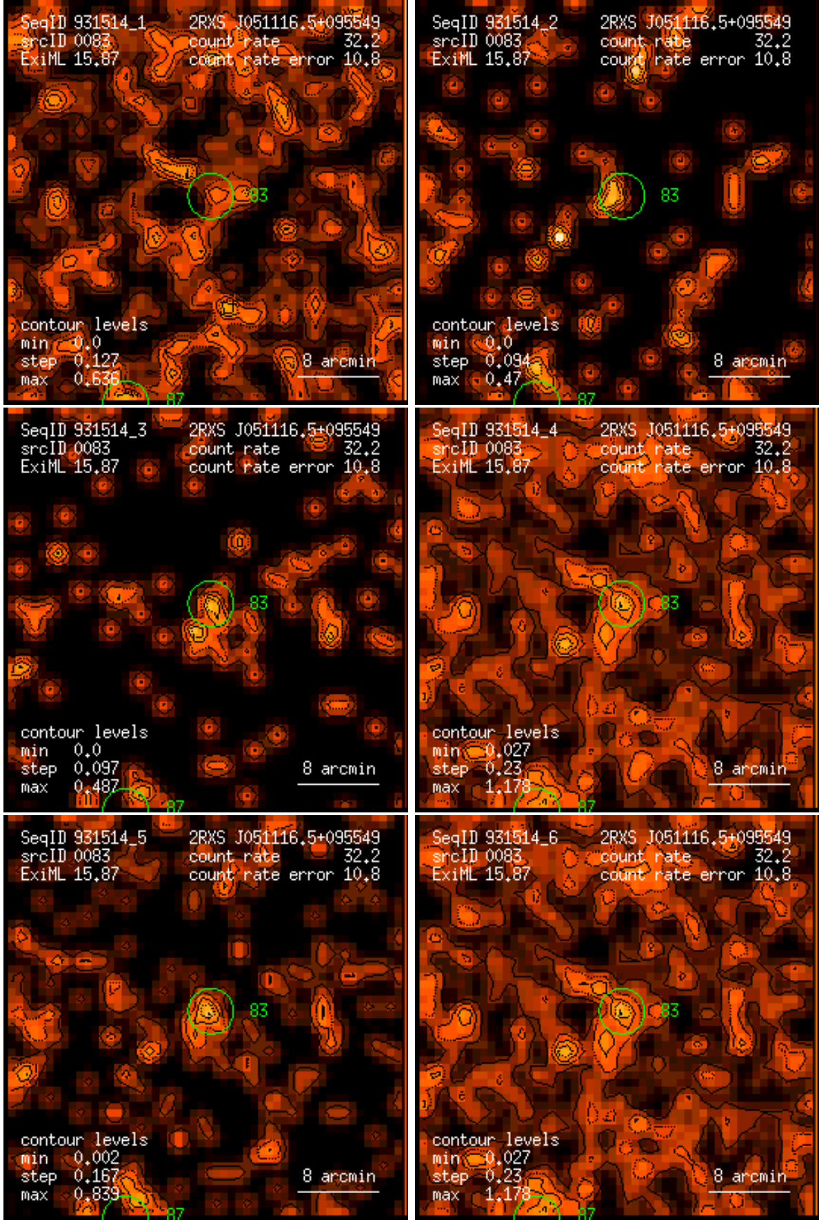
Figure 83: RASS 931514: detection 0083: band rate images, Gaussian filter: (1) PSPC channels 11 – 41, (2) 52 – 90, (3) 91 – 201, (4) 11 – 235, (5) 52 – 201, (6) 11 – 201. Broad band rates in counts/ks. Band rate contour levels in counts/ks/arcmin 2 .
