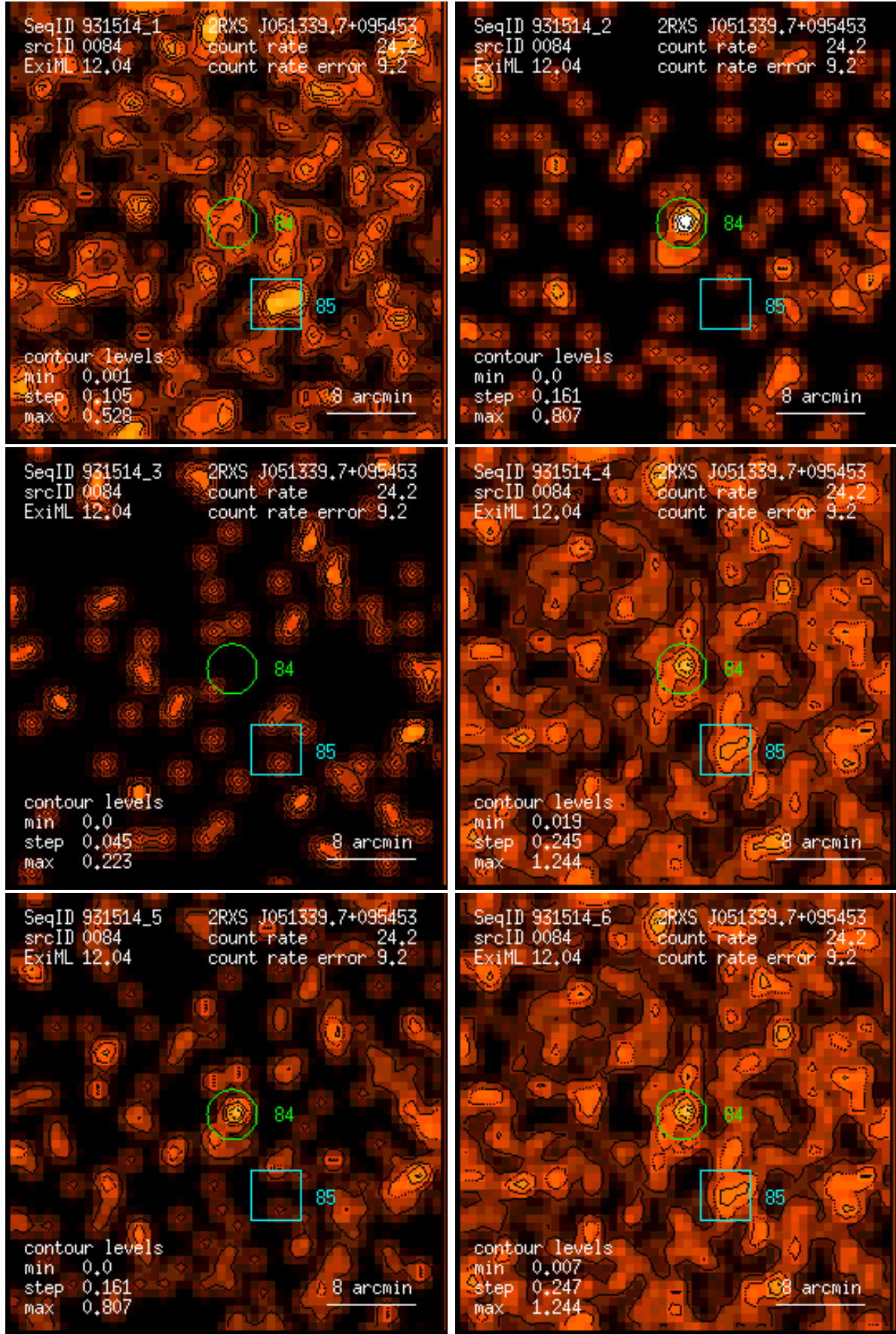
Figure 84: RASS 931514: detection 0084: band rate images, Gaussian filter: (1) PSPC channels 11 – 41, (2) 52 – 90, (3) 91 – 201, (4) 11 – 235, (5) 52 – 201, (6) 11 – 201. Broad band rates in counts/ks. Band rate contour levels in counts/ks/arcmin 2 .
