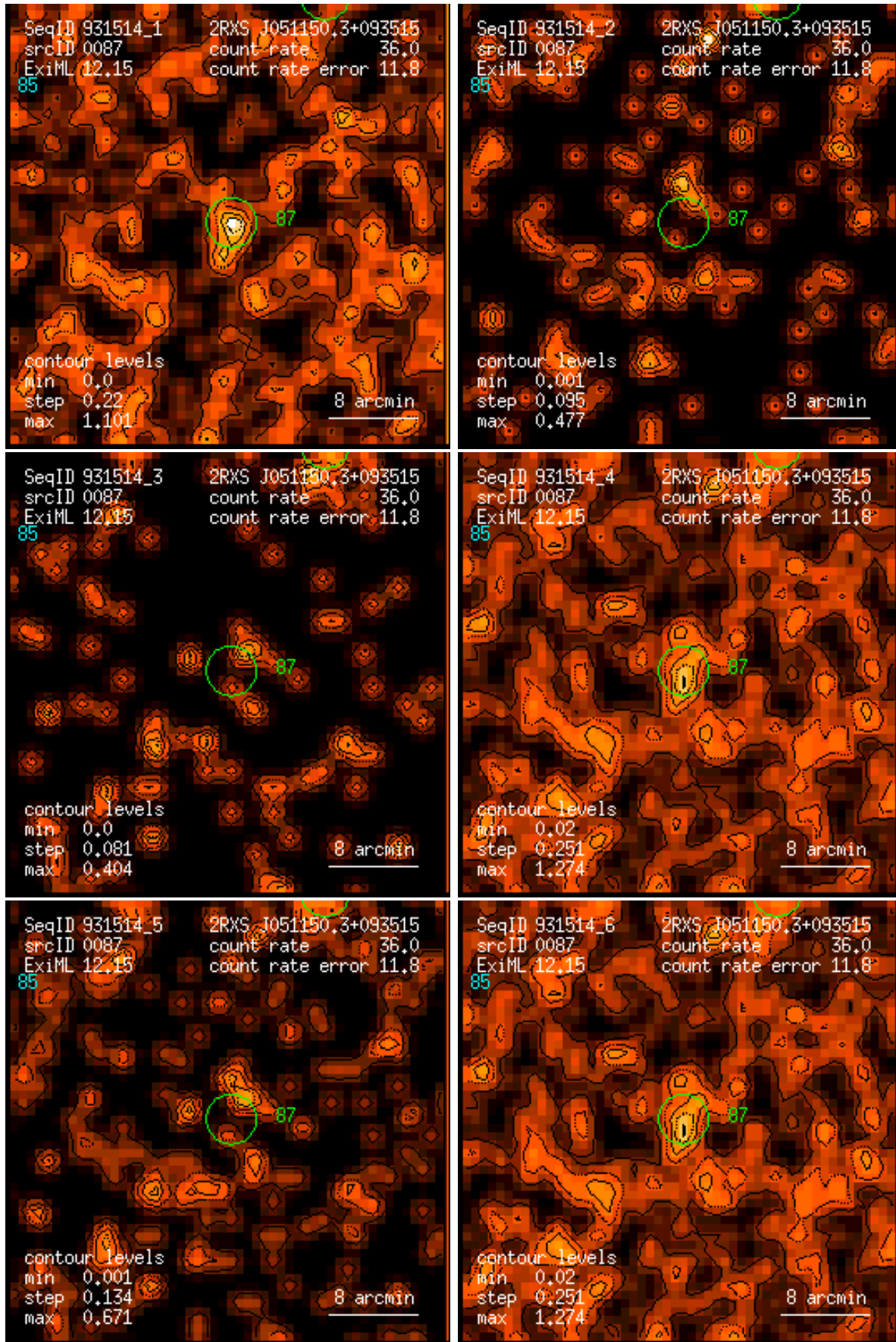
Figure 87: RASS 931514: detection 0087: band rate images, Gaussian filter: (1) PSPC channels 11 – 41, (2) 52 – 90, (3) 91 – 201, (4) 11 – 235, (5) 52 – 201, (6) 11 – 201. Broad band rates in counts/ks. Band rate contour levels in counts/ks/arcmin 2 .
