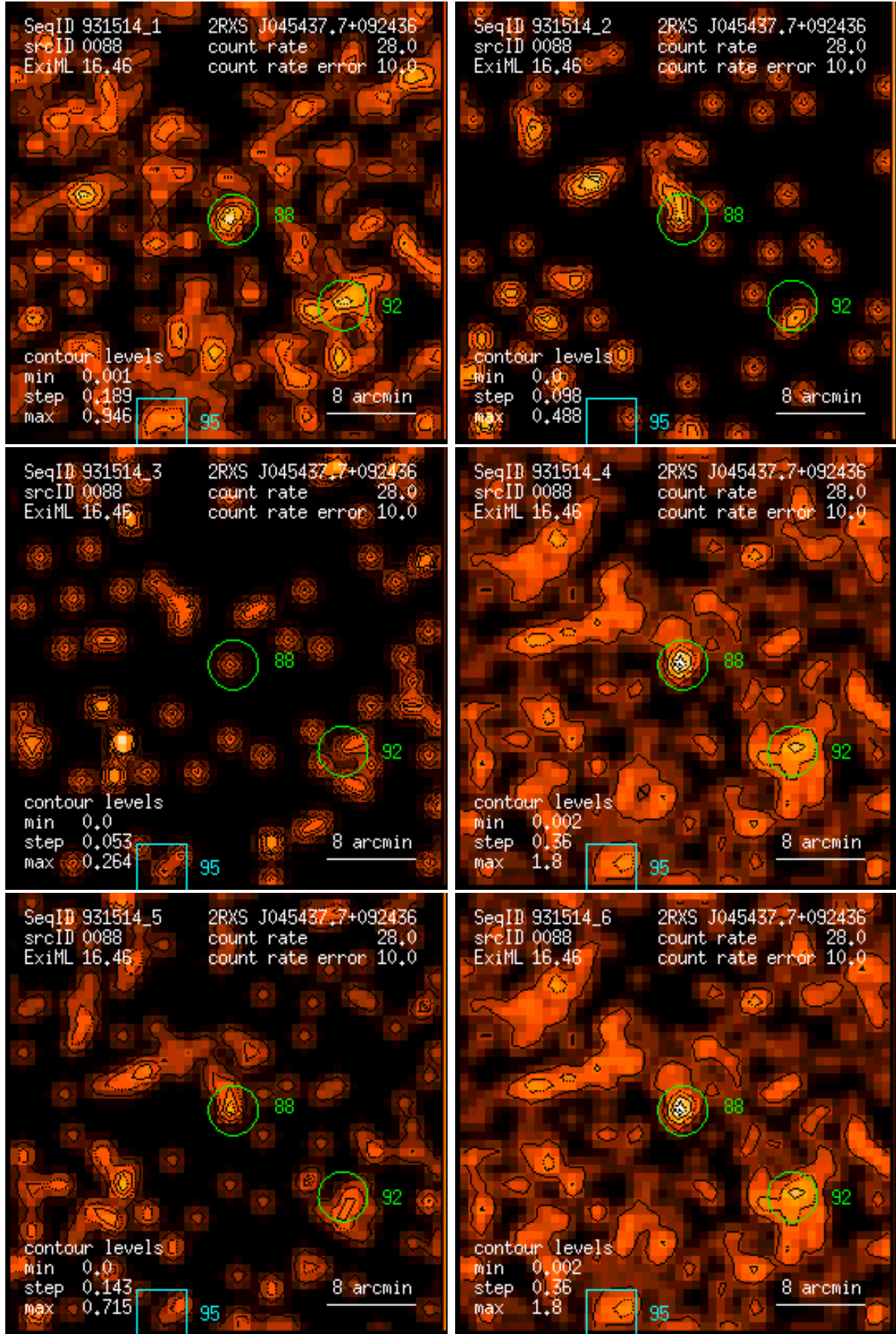
Figure 88: RASS 931514: detection 0088: band rate images, Gaussian filter: (1) PSPC channels 11 – 41, (2) 52 – 90, (3) 91 – 201, (4) 11 – 235, (5) 52 – 201, (6) 11 – 201. Broad band rates in counts/ks. Band rate contour levels in counts/ks/arcmin 2 .
