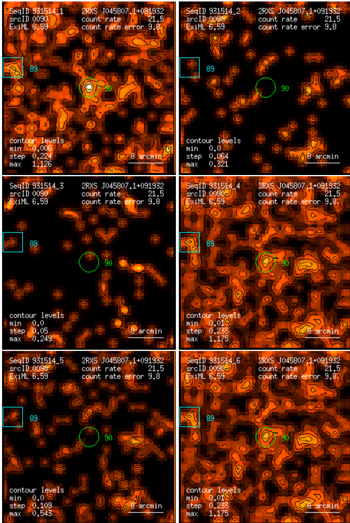
Figure 90: RASS 931514: detection 0090: band rate images, Gaussian filter: (1) PSPC channels 11 – 41, (2) 52 – 90, (3) 91 – 201, (4) 11 – 235, (5) 52 – 201, (6) 11 – 201. Broad band rates in counts/ks. Band rate contour levels in counts/ks/arcmin 2 .
