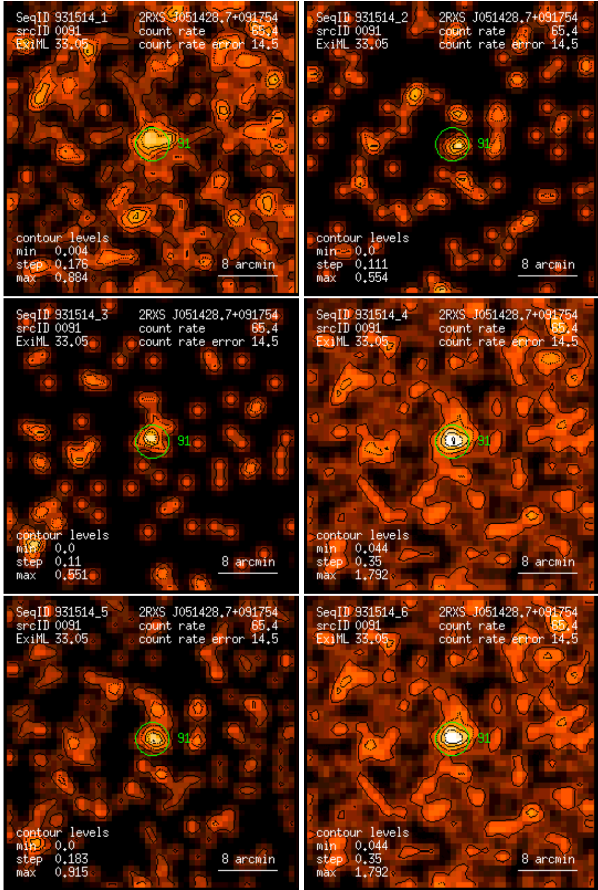
Figure 91: RASS 931514: detection 0091: band rate images, Gaussian filter: (1) PSPC channels 11 – 41, (2) 52 – 90, (3) 91 – 201, (4) 11 – 235, (5) 52 – 201, (6) 11 – 201. Broad band rates in counts/ks. Band rate contour levels in counts/ks/arcmin 2 .
