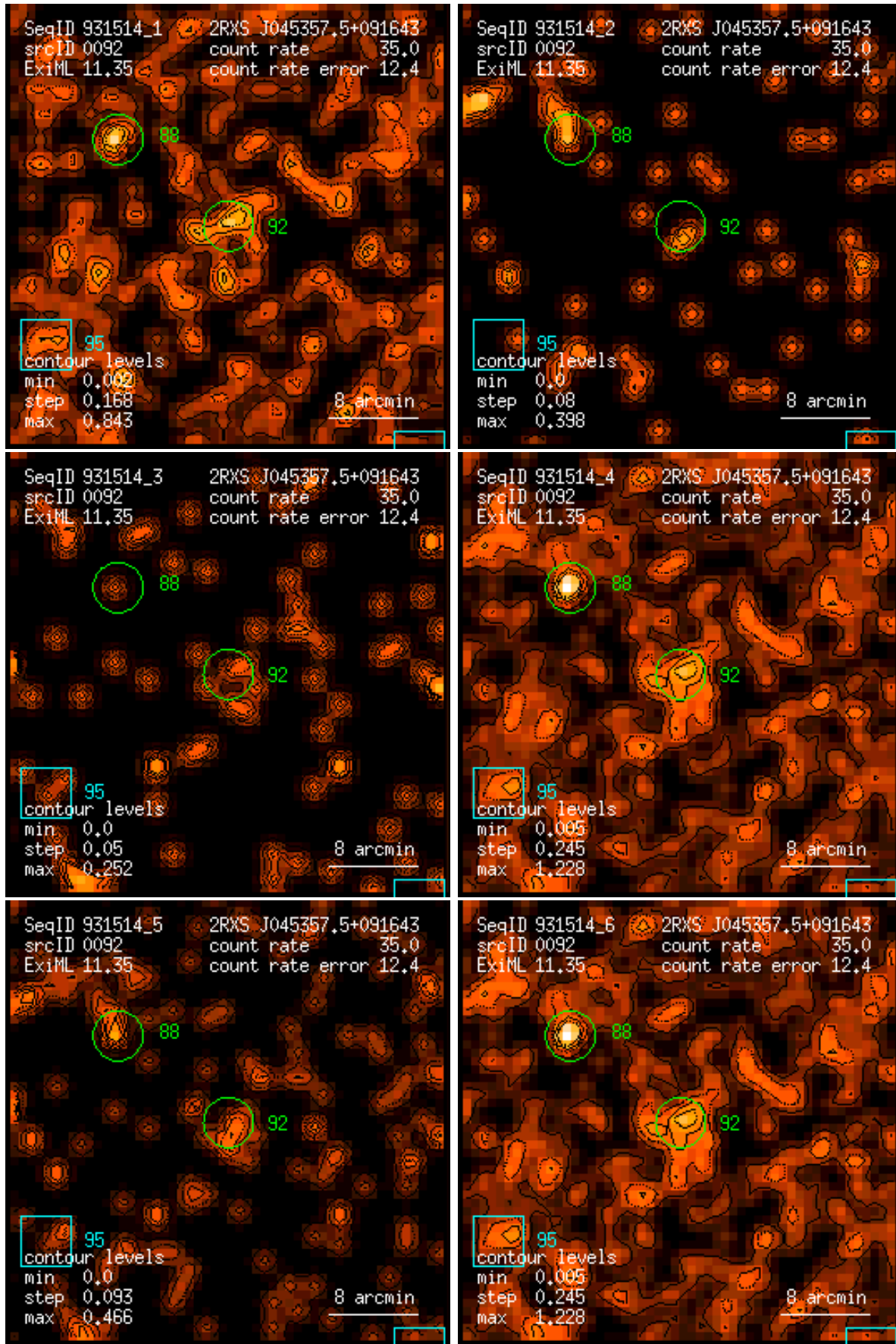
Figure 92: RASS 931514: detection 0092: band rate images, Gaussian filter: (1) PSPC channels 11 – 41, (2) 52 – 90, (3) 91 – 201, (4) 11 – 235, (5) 52 – 201, (6) 11 – 201. Broad band rates in counts/ks. Band rate contour levels in counts/ks/arcmin 2 .
