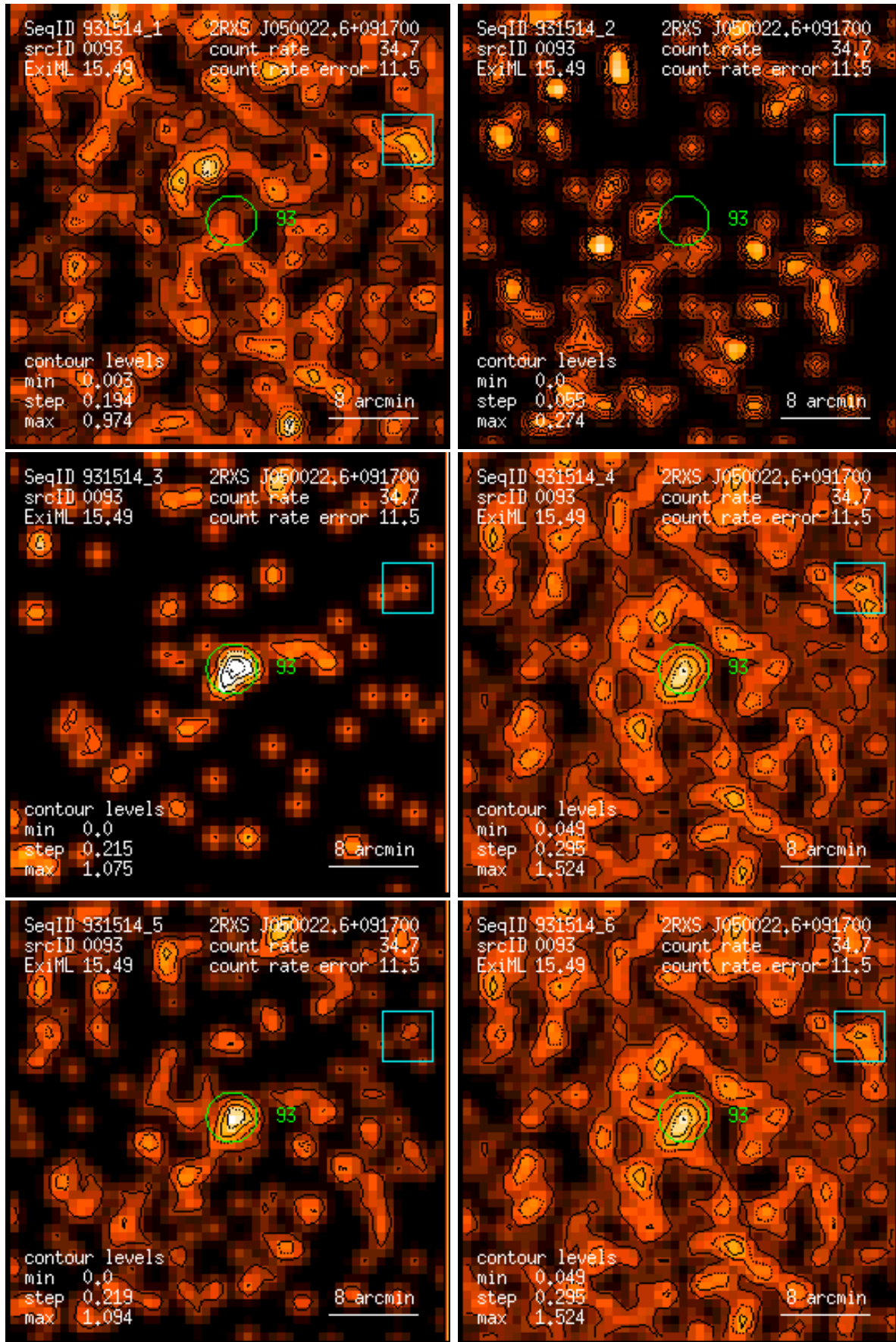
Figure 93: RASS 931514: detection 0093: band rate images, Gaussian filter: (1) PSPC channels 11 – 41, (2) 52 – 90, (3) 91 – 201, (4) 11 – 235, (5) 52 – 201, (6) 11 – 201. Broad band rates in counts/ks. Band rate contour levels in counts/ks/arcmin 2 .
