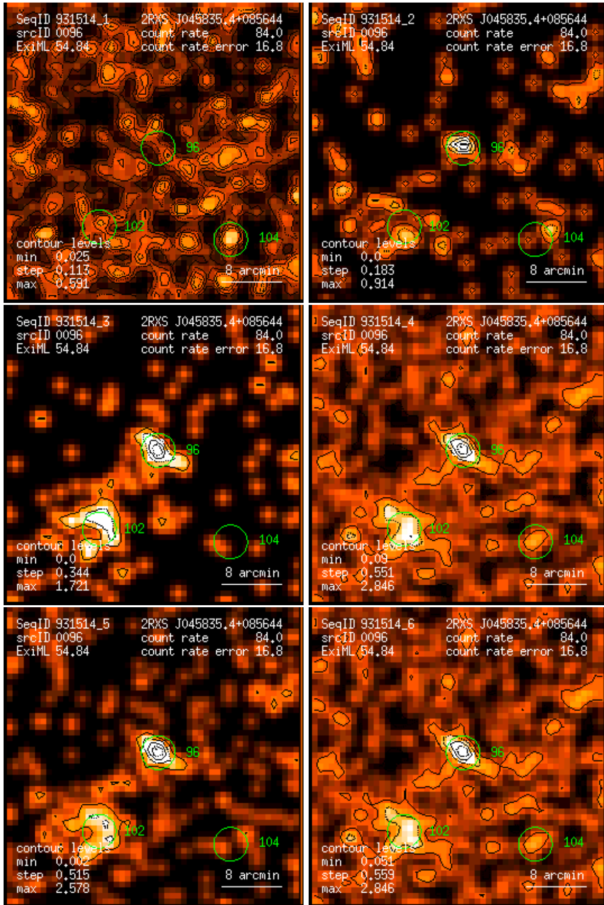
Figure 96: RASS 931514: detection 0096: band rate images, Gaussian filter: (1) PSPC channels 11 – 41, (2) 52 – 90, (3) 91 – 201, (4) 11 – 235, (5) 52 – 201, (6) 11 – 201. Broad band rates in counts/ks. Band rate contour levels in counts/ks/arcmin 2 .
