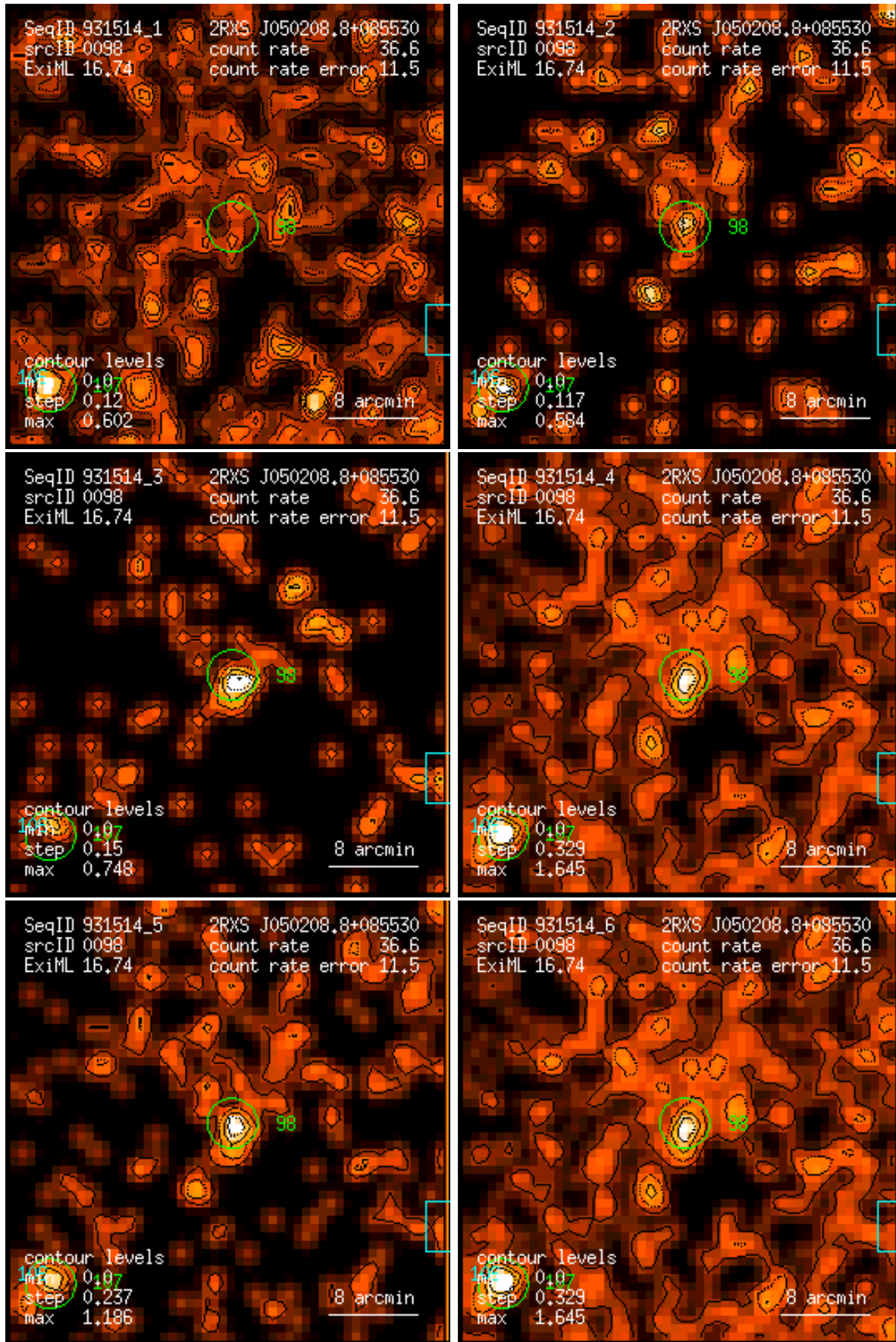
Figure 98: RASS 931514: detection 0098: band rate images, Gaussian filter: (1) PSPC channels 11 – 41, (2) 52 – 90, (3) 91 – 201, (4) 11 – 235, (5) 52 – 201, (6) 11 – 201. Broad band rates in counts/ks. Band rate contour levels in counts/ks/arcmin 2 .
