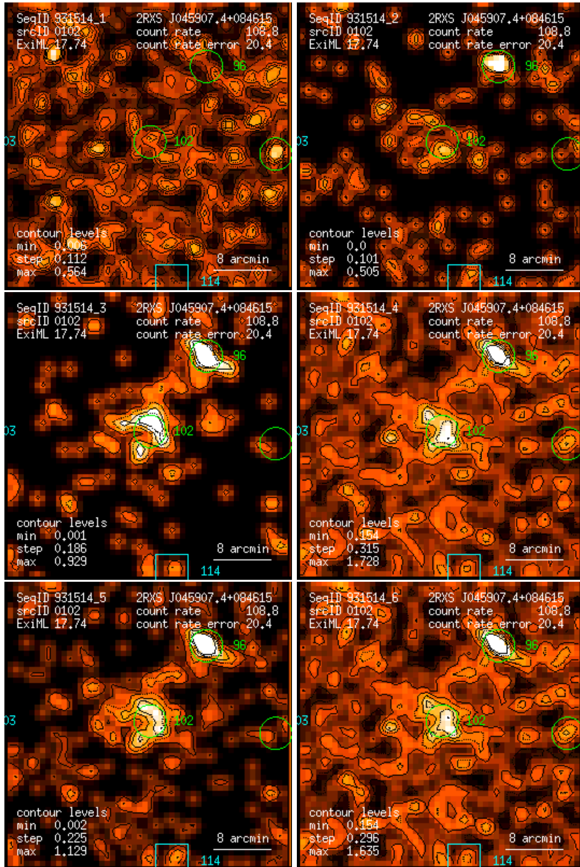
Figure 102: RASS 931514: detection 0102: band rate images, Gaussian filter: (1) PSPC channels 11 – 41, (2) 52 – 90, (3) 91 – 201, (4) 11 – 235, (5) 52 – 201, (6) 11 – 201. Broad band rates in counts/ks. Band rate contour levels in counts/ks/arcmin 2 .
