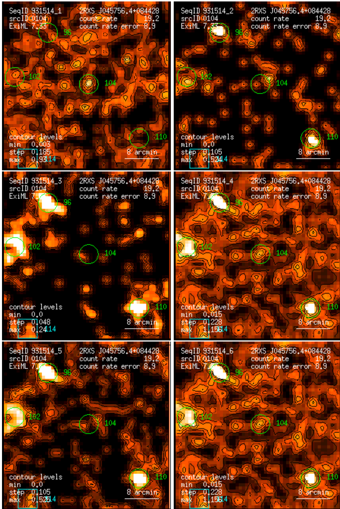
Figure 104: RASS 931514: detection 0104: band rate images, Gaussian filter: (1) PSPC channels 11 – 41, (2) 52 – 90, (3) 91 – 201, (4) 11 – 235, (5) 52 – 201, (6) 11 – 201. Broad band rates in counts/ks. Band rate contour levels in counts/ks/arcmin 2 .
