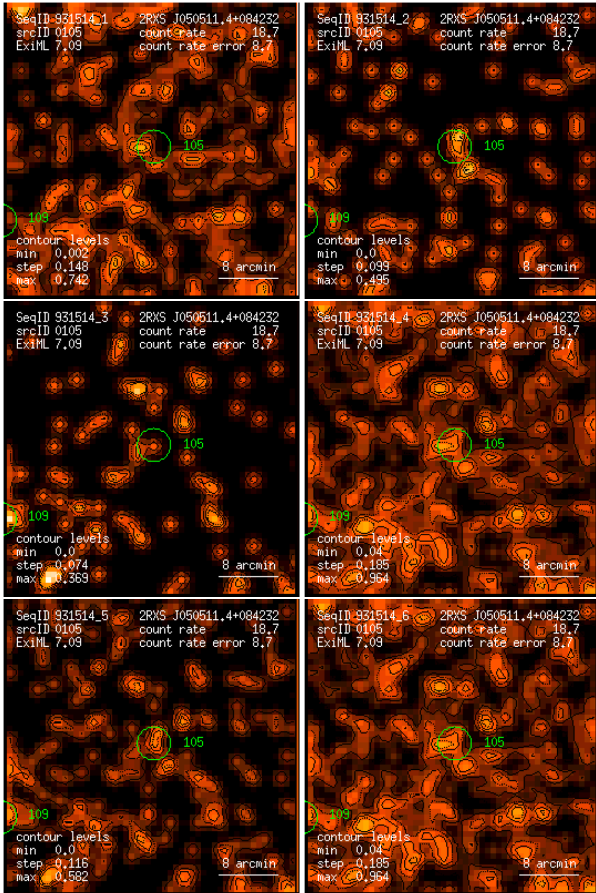
Figure 105: RASS 931514: detection 0105: band rate images, Gaussian filter: (1) PSPC channels 11 – 41, (2) 52 – 90, (3) 91 – 201, (4) 11 – 235, (5) 52 – 201, (6) 11 – 201. Broad band rates in counts/ks. Band rate contour levels in counts/ks/arcmin 2 .
