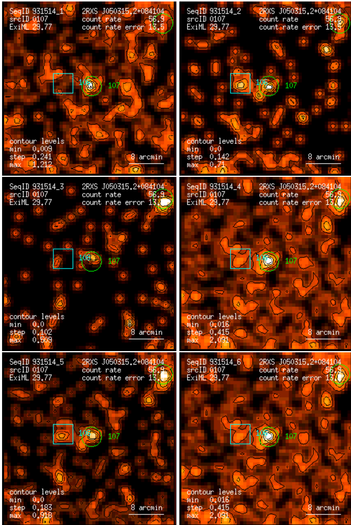
Figure 107: RASS 931514: detection 0107: band rate images, Gaussian filter: (1) PSPC channels 11 – 41, (2) 52 – 90, (3) 91 – 201, (4) 11 – 235, (5) 52 – 201, (6) 11 – 201. Broad band rates in counts/ks. Band rate contour levels in counts/ks/arcmin 2 .
