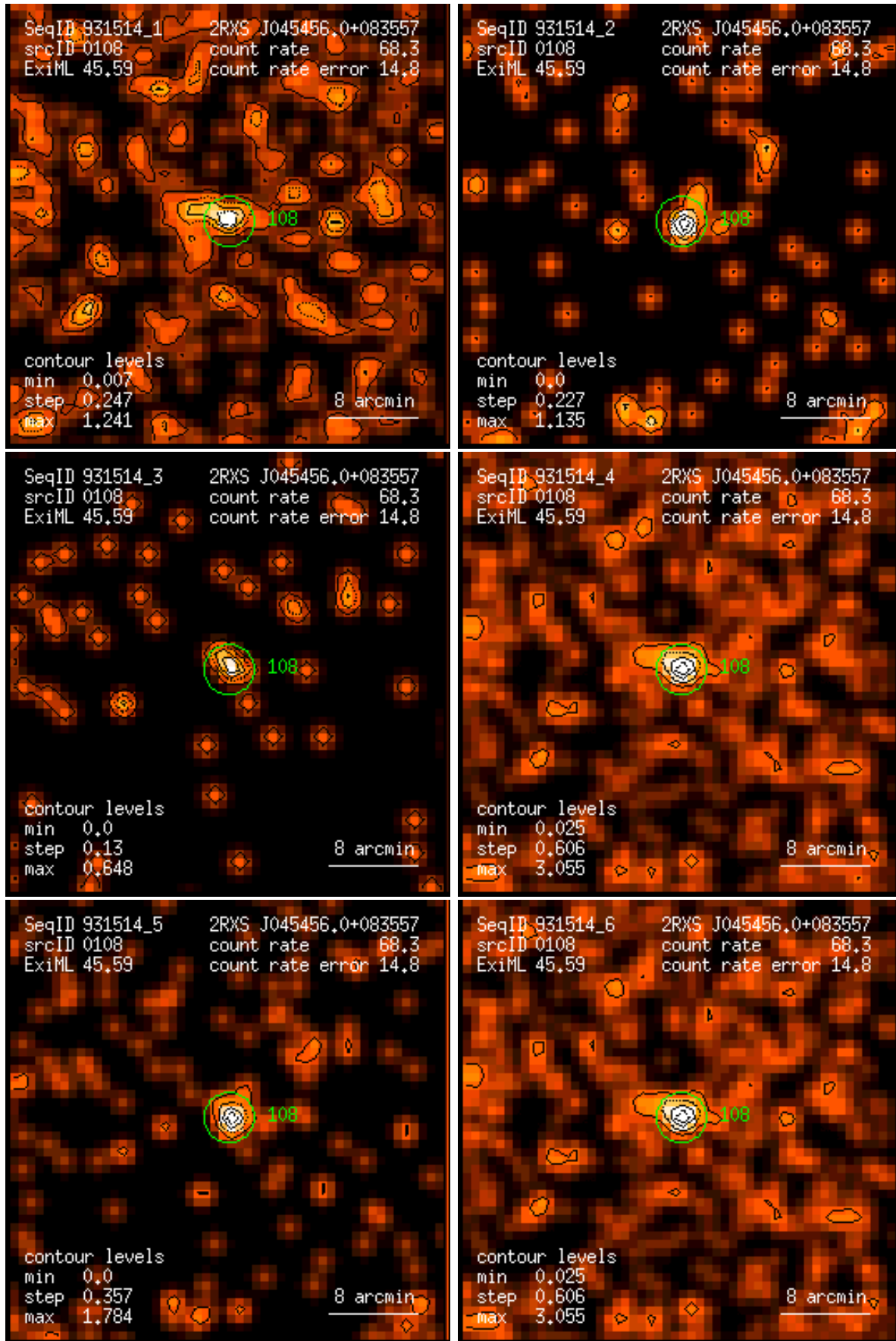
Figure 108: RASS 931514: detection 0108: band rate images, Gaussian filter: (1) PSPC channels 11 – 41, (2) 52 – 90, (3) 91 – 201, (4) 11 – 235, (5) 52 – 201, (6) 11 – 201. Broad band rates in counts/ks. Band rate contour levels in counts/ks/arcmin 2 .
